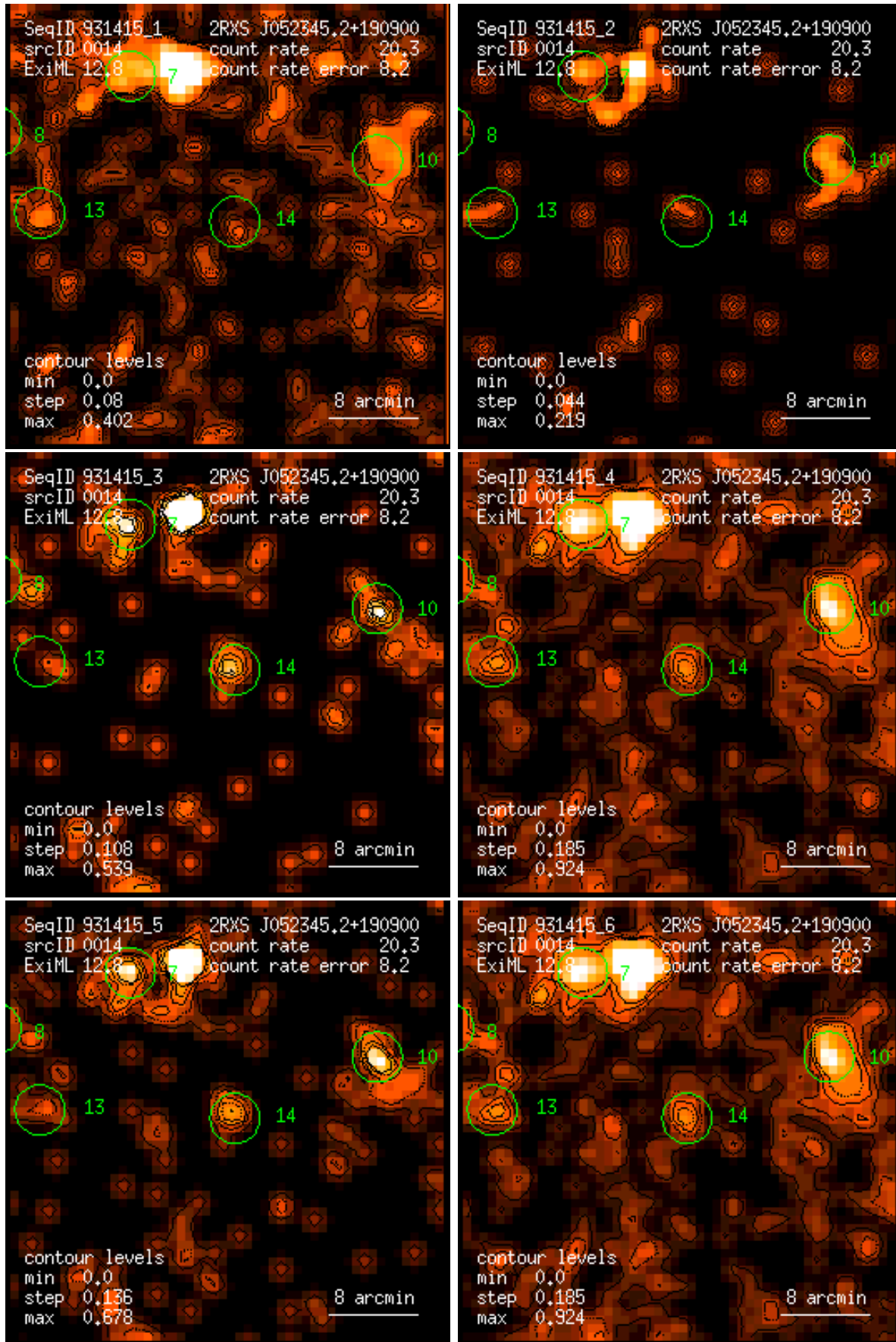
Figure 14: RASS 931415: detection 0014: band rate images, Gaussian filter: (1) PSPC channels 11 – 41, (2) 52 – 90, (3) 91 – 201, (4) 11 – 235, (5) 52 – 201, (6) 11 – 201. Broad band rates in counts/ks. Band rate contour levels in counts/ks/arcmin 2 .
