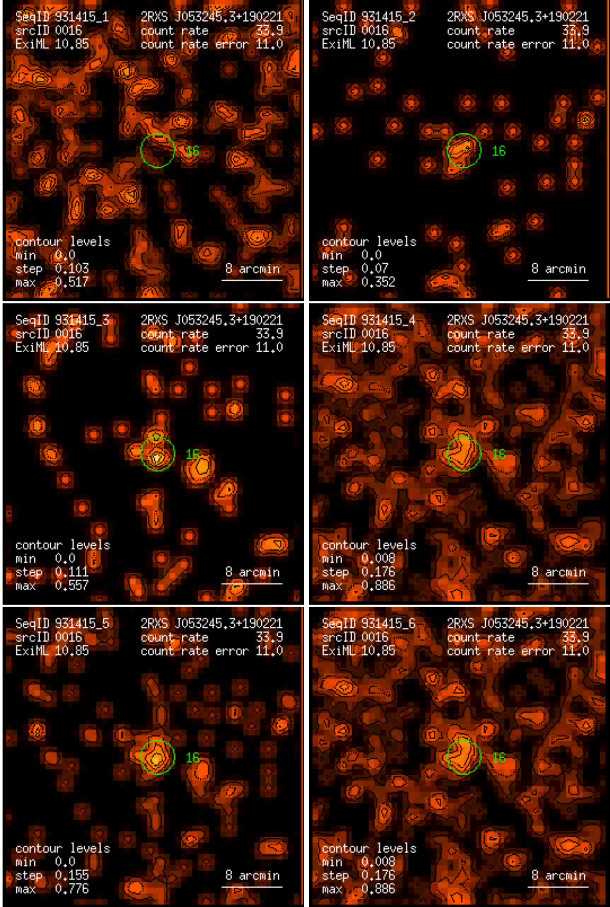
Figure 16: RASS 931415: detection 0016: band rate images, Gaussian filter: (1) PSPC channels 11 – 41, (2) 52 – 90, (3) 91 – 201, (4) 11 – 235, (5) 52 – 201, (6) 11 – 201. Broad band rates in counts/ks. Band rate contour levels in counts/ks/arcmin 2 .
