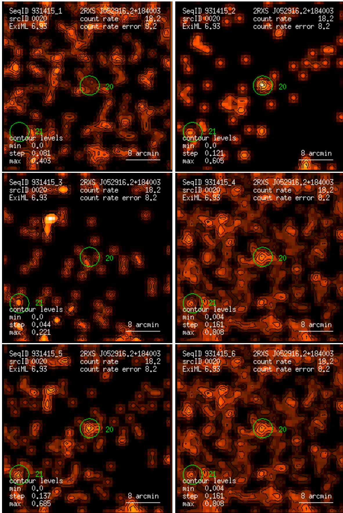
Figure 20: RASS 931415: detection 0020: band rate images, Gaussian filter: (1) PSPC channels 11 – 41, (2) 52 – 90, (3) 91 – 201, (4) 11 – 235, (5) 52 – 201, (6) 11 – 201. Broad band rates in counts/ks. Band rate contour levels in counts/ks/arcmin 2 .
