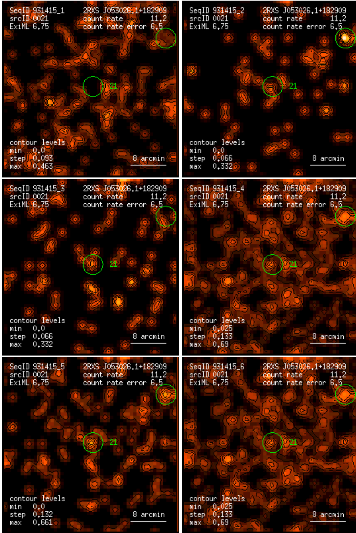
Figure 21: RASS 931415: detection 0021: band rate images, Gaussian filter: (1) PSPC channels 11 – 41, (2) 52 – 90, (3) 91 – 201, (4) 11 – 235, (5) 52 – 201, (6) 11 – 201. Broad band rates in counts/ks. Band rate contour levels in counts/ks/arcmin 2 .
