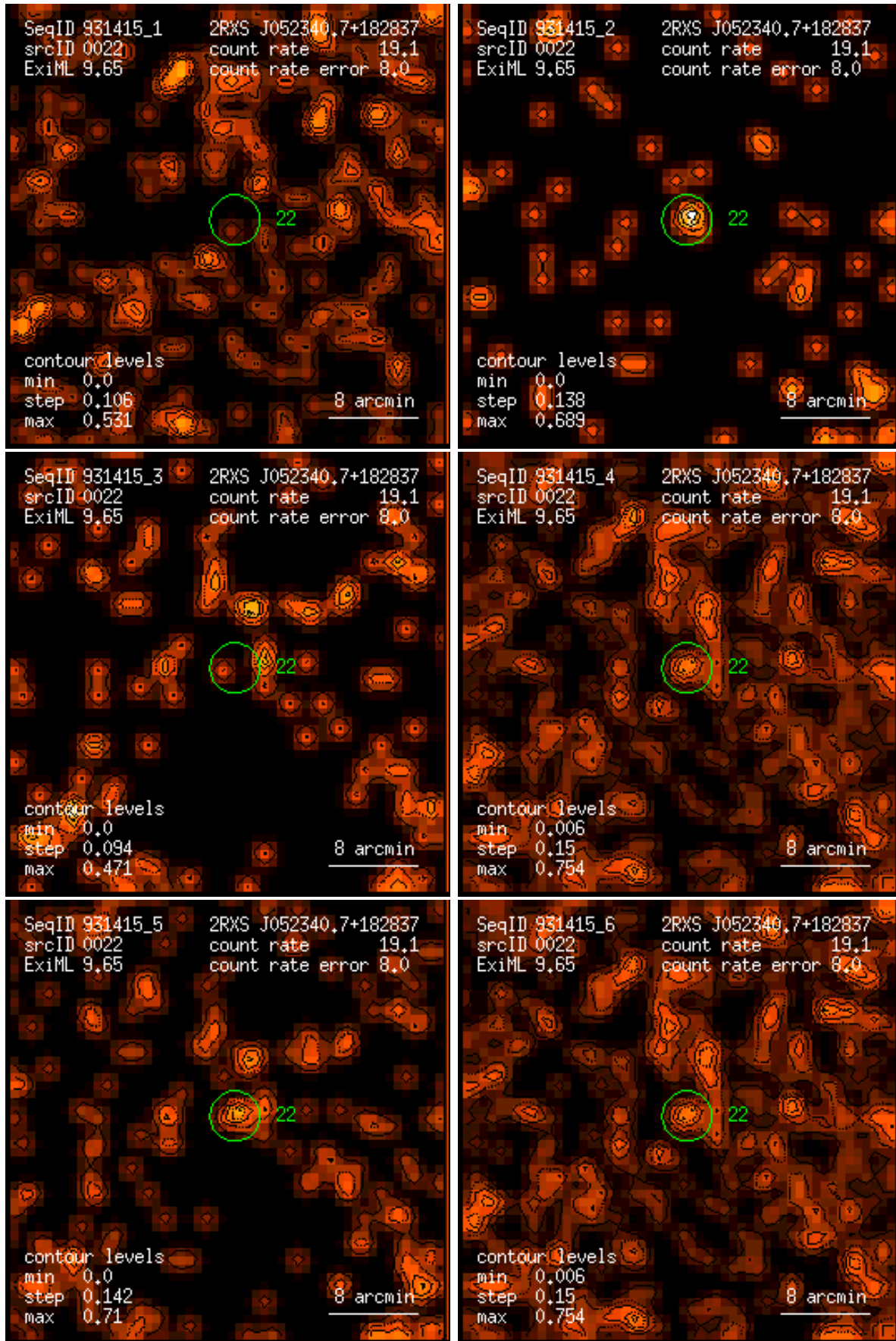
Figure 22: RASS 931415: detection 0022: band rate images, Gaussian filter: (1) PSPC channels 11 – 41, (2) 52 – 90, (3) 91 – 201, (4) 11 – 235, (5) 52 – 201, (6) 11 – 201. Broad band rates in counts/ks. Band rate contour levels in counts/ks/arcmin 2 .
