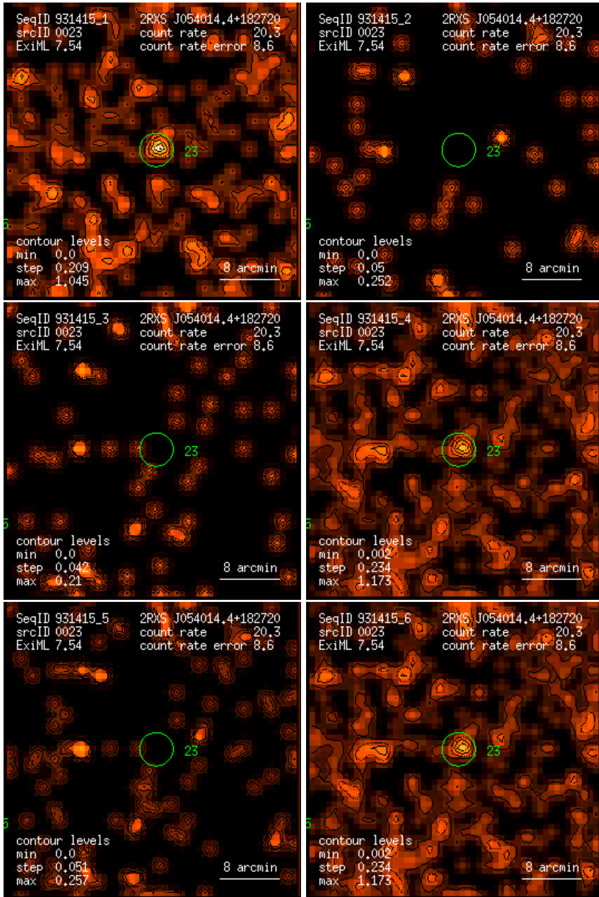
Figure 23: RASS 931415: detection 0023: band rate images, Gaussian filter: (1) PSPC channels 11 – 41, (2) 52 – 90, (3) 91 – 201, (4) 11 – 235, (5) 52 – 201, (6) 11 – 201. Broad band rates in counts/ks. Band rate contour levels in counts/ks/arcmin 2 .
