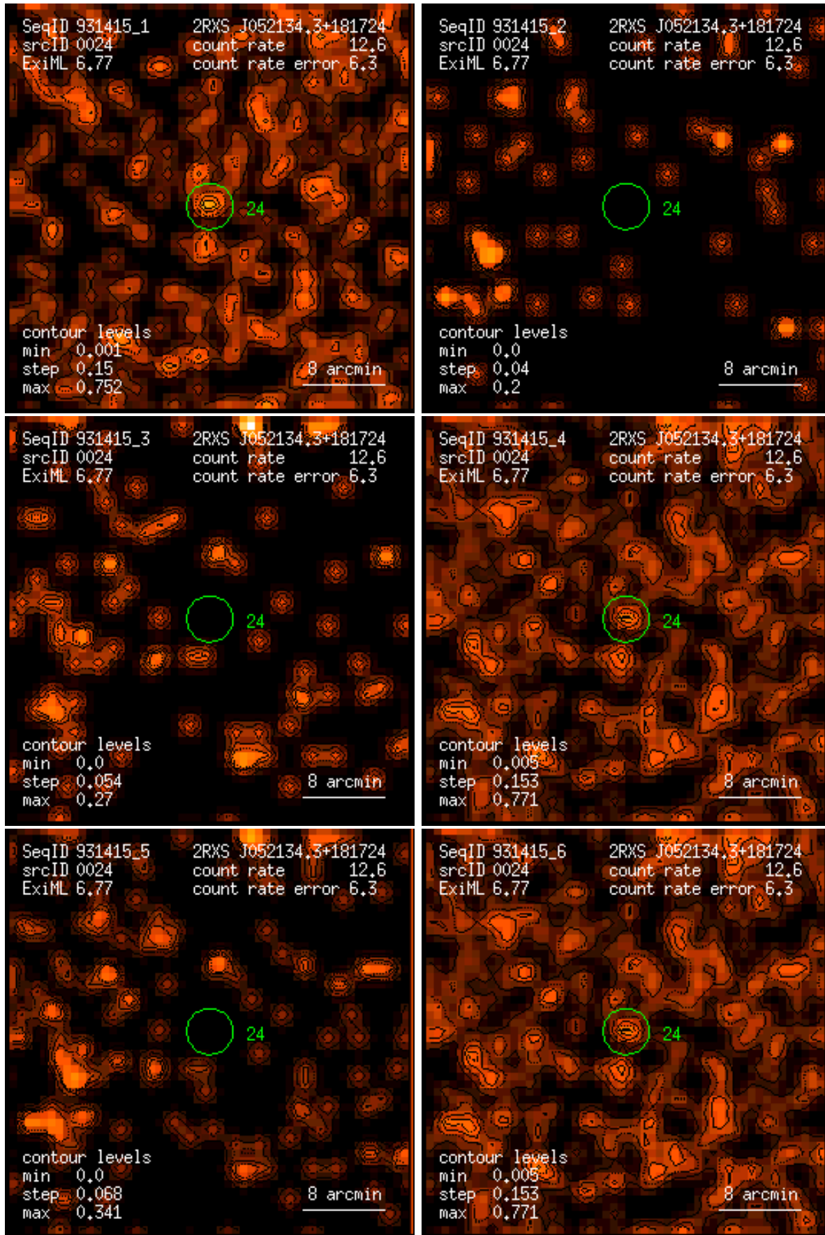
Figure 24: RASS 931415: detection 0024: band rate images, Gaussian filter: (1) PSPC channels 11 – 41, (2) 52 – 90, (3) 91 – 201, (4) 11 – 235, (5) 52 – 201, (6) 11 – 201. Broad band rates in counts/ks. Band rate contour levels in counts/ks/arcmin 2 .
