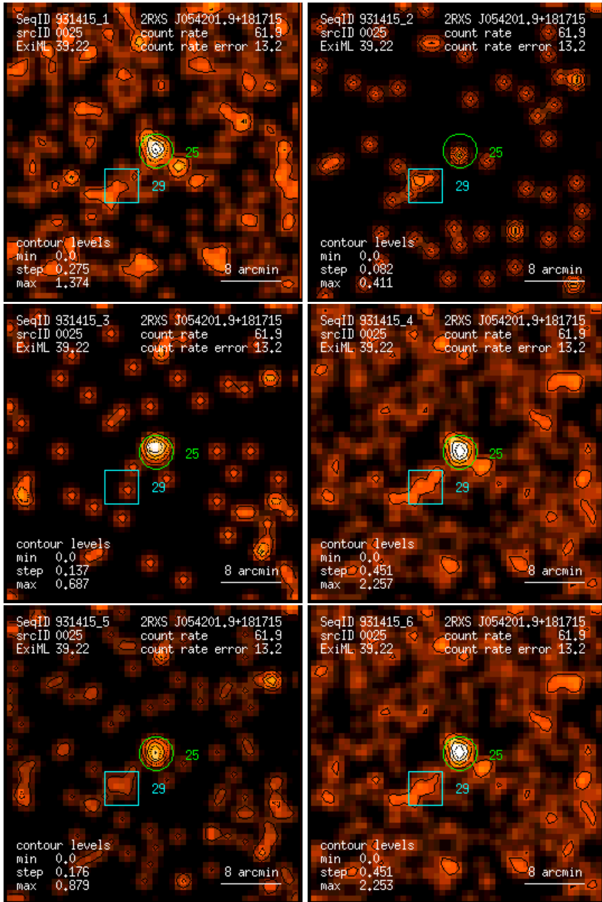
Figure 25: RASS 931415: detection 0025: band rate images, Gaussian filter: (1) PSPC channels 11 – 41, (2) 52 – 90, (3) 91 – 201, (4) 11 – 235, (5) 52 – 201, (6) 11 – 201. Broad band rates in counts/ks. Band rate contour levels in counts/ks/arcmin 2 .
