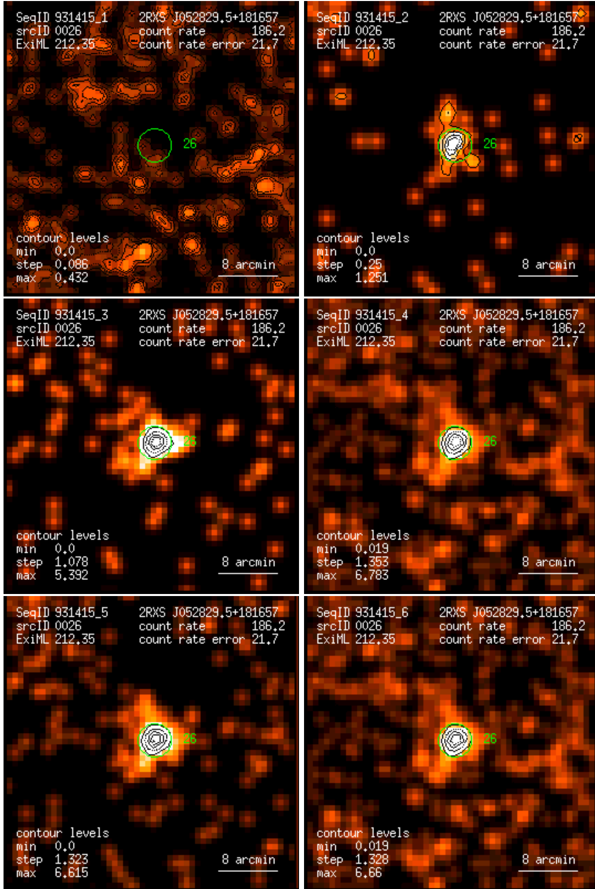
Figure 26: RASS 931415: detection 0026: band rate images, Gaussian filter: (1) PSPC channels 11 – 41, (2) 52 – 90, (3) 91 – 201, (4) 11 – 235, (5) 52 – 201, (6) 11 – 201. Broad band rates in counts/ks. Band rate contour levels in counts/ks/arcmin 2 .
