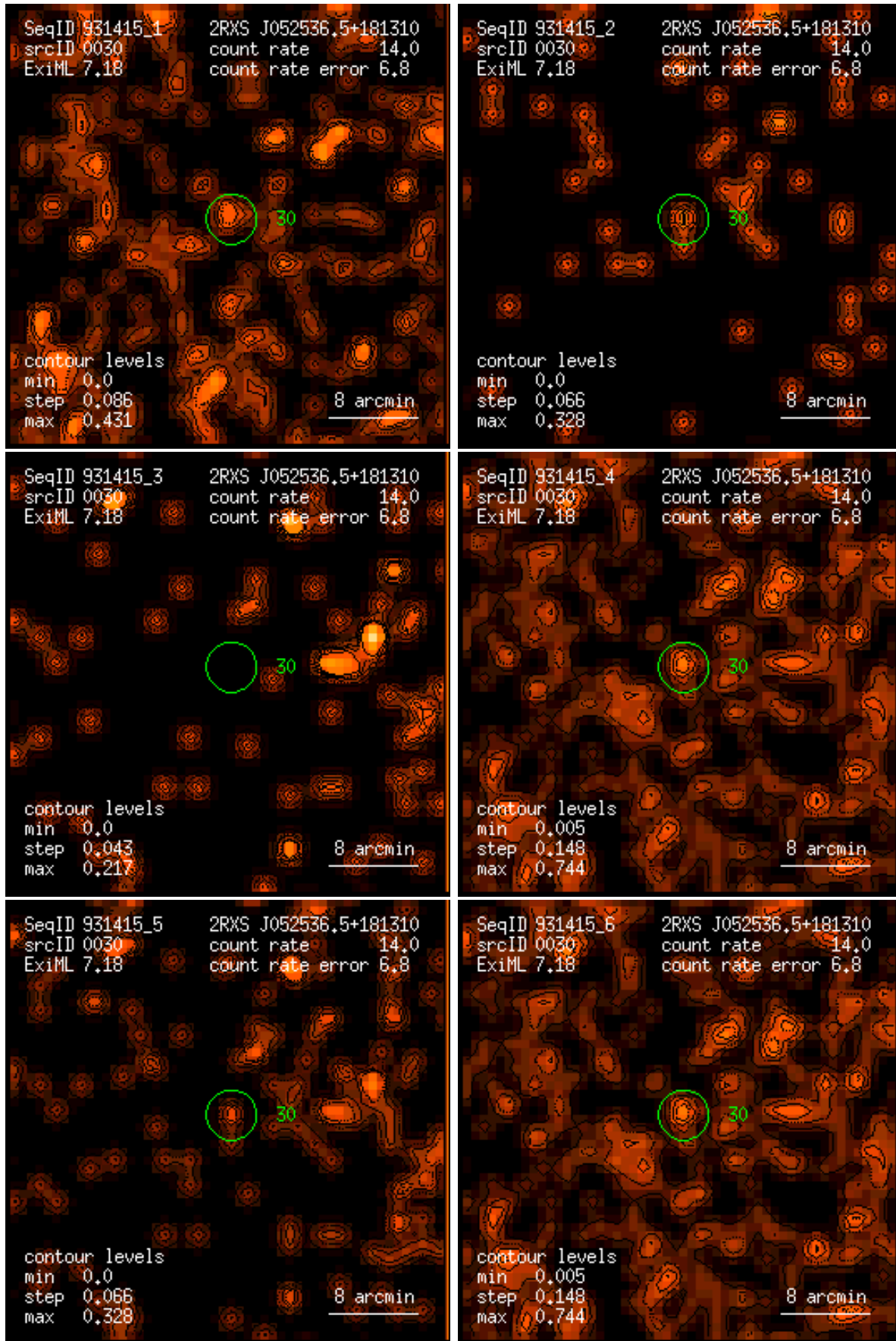
Figure 30: RASS 931415: detection 0030: band rate images, Gaussian filter: (1) PSPC channels 11 – 41, (2) 52 – 90, (3) 91 – 201, (4) 11 – 235, (5) 52 – 201, (6) 11 – 201. Broad band rates in counts/ks. Band rate contour levels in counts/ks/arcmin 2 .
