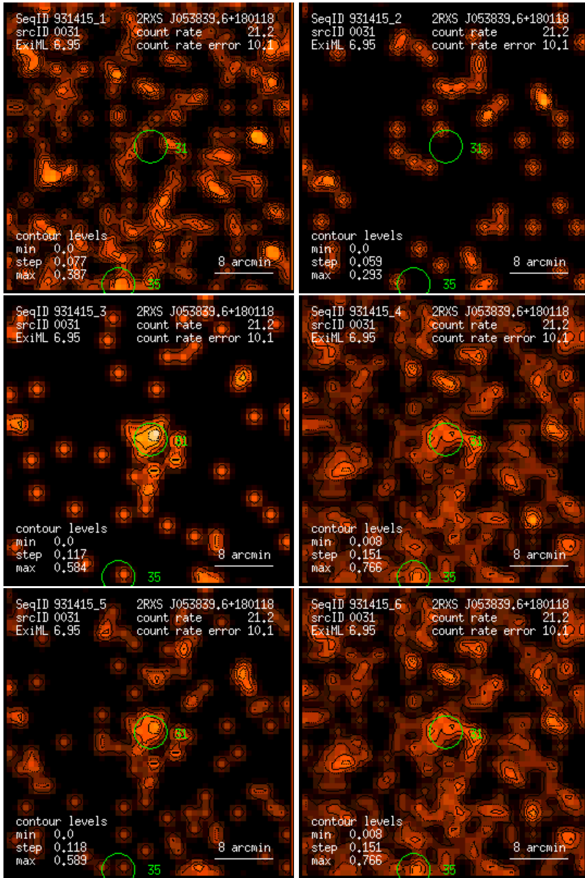
Figure 31: RASS 931415: detection 0031: band rate images, Gaussian filter: (1) PSPC channels 11 – 41, (2) 52 – 90, (3) 91 – 201, (4) 11 – 235, (5) 52 – 201, (6) 11 – 201. Broad band rates in counts/ks. Band rate contour levels in counts/ks/arcmin 2 .
