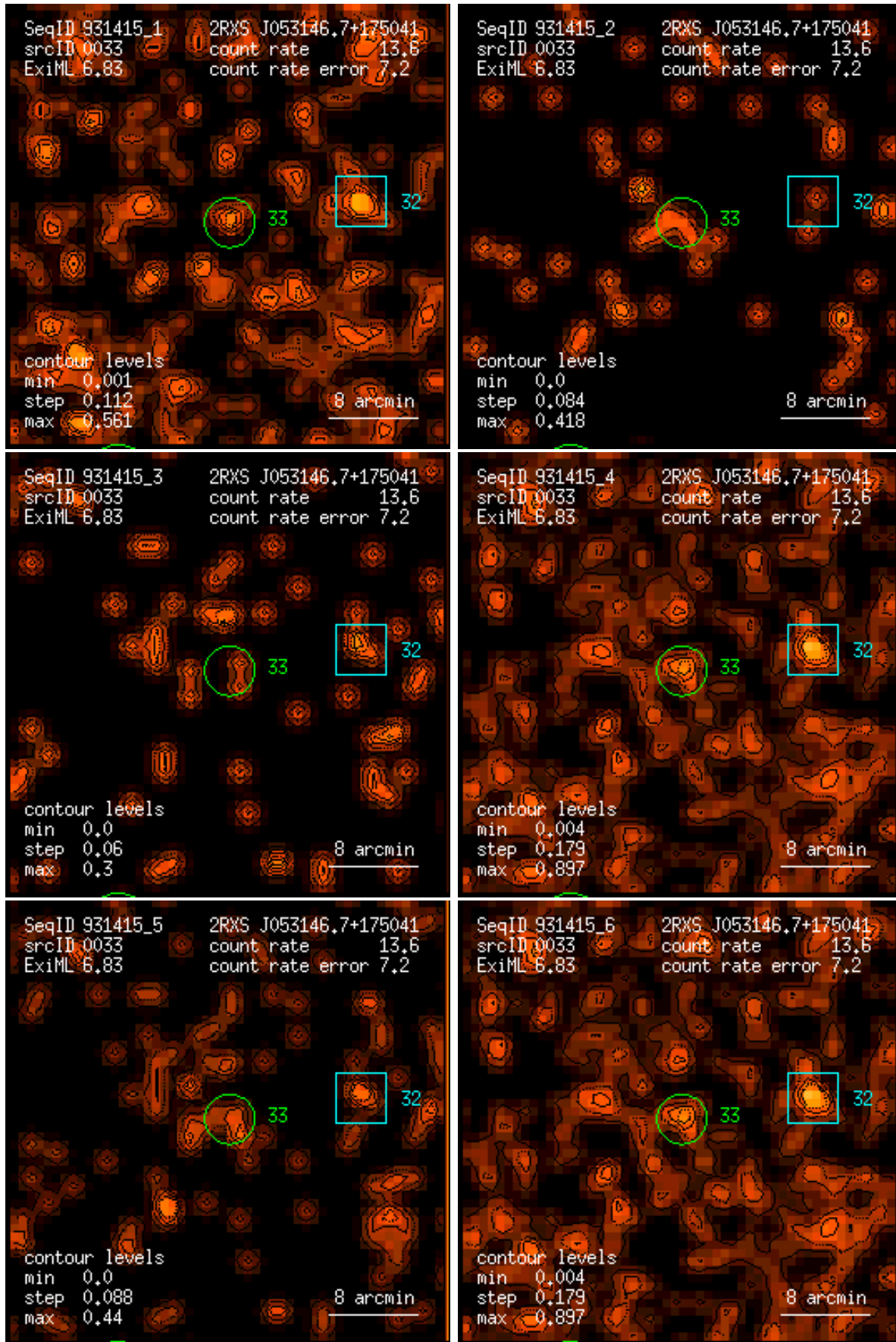
Figure 33: RASS 931415: detection 0033: band rate images, Gaussian filter: (1) PSPC channels 11 – 41, (2) 52 – 90, (3) 91 – 201, (4) 11 – 235, (5) 52 – 201, (6) 11 – 201. Broad band rates in counts/ks. Band rate contour levels in counts/ks/arcmin 2 .
