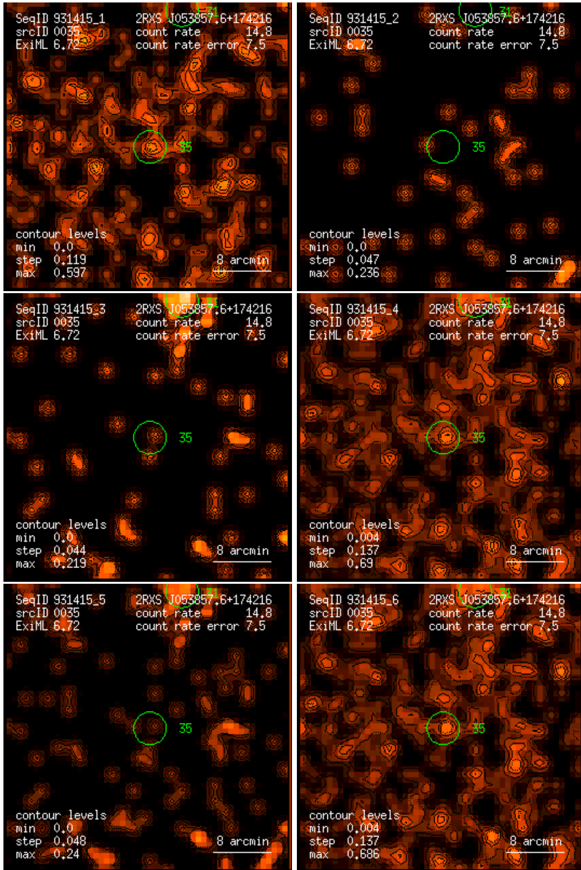
Figure 35: RASS 931415: detection 0035: band rate images, Gaussian filter: (1) PSPC channels 11 – 41, (2) 52 – 90, (3) 91 – 201, (4) 11 – 235, (5) 52 – 201, (6) 11 – 201. Broad band rates in counts/ks. Band rate contour levels in counts/ks/arcmin 2 .
