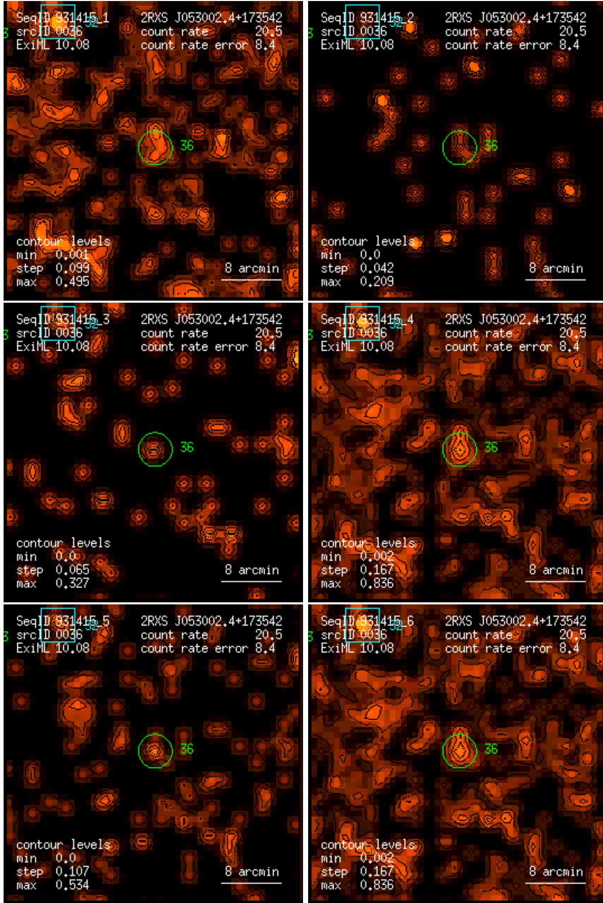
Figure 36: RASS 931415: detection 0036: band rate images, Gaussian filter: (1) PSPC channels 11 – 41, (2) 52 – 90, (3) 91 – 201, (4) 11 – 235, (5) 52 – 201, (6) 11 – 201. Broad band rates in counts/ks. Band rate contour levels in counts/ks/arcmin 2 .
