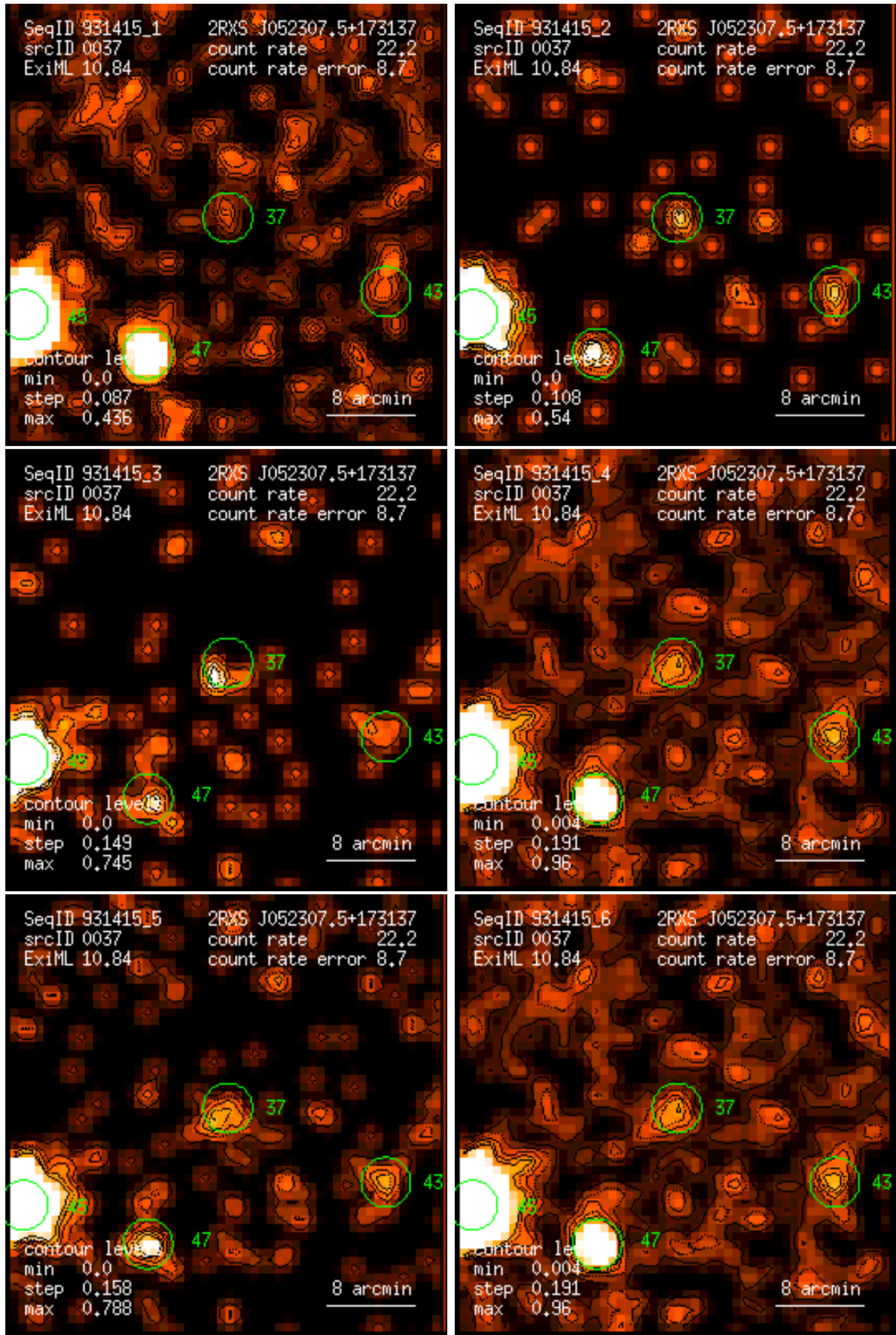
Figure 37: RASS 931415: detection 0037: band rate images, Gaussian filter: (1) PSPC channels 11 – 41, (2) 52 – 90, (3) 91 – 201, (4) 11 – 235, (5) 52 – 201, (6) 11 – 201. Broad band rates in counts/ks. Band rate contour levels in counts/ks/arcmin 2 .
