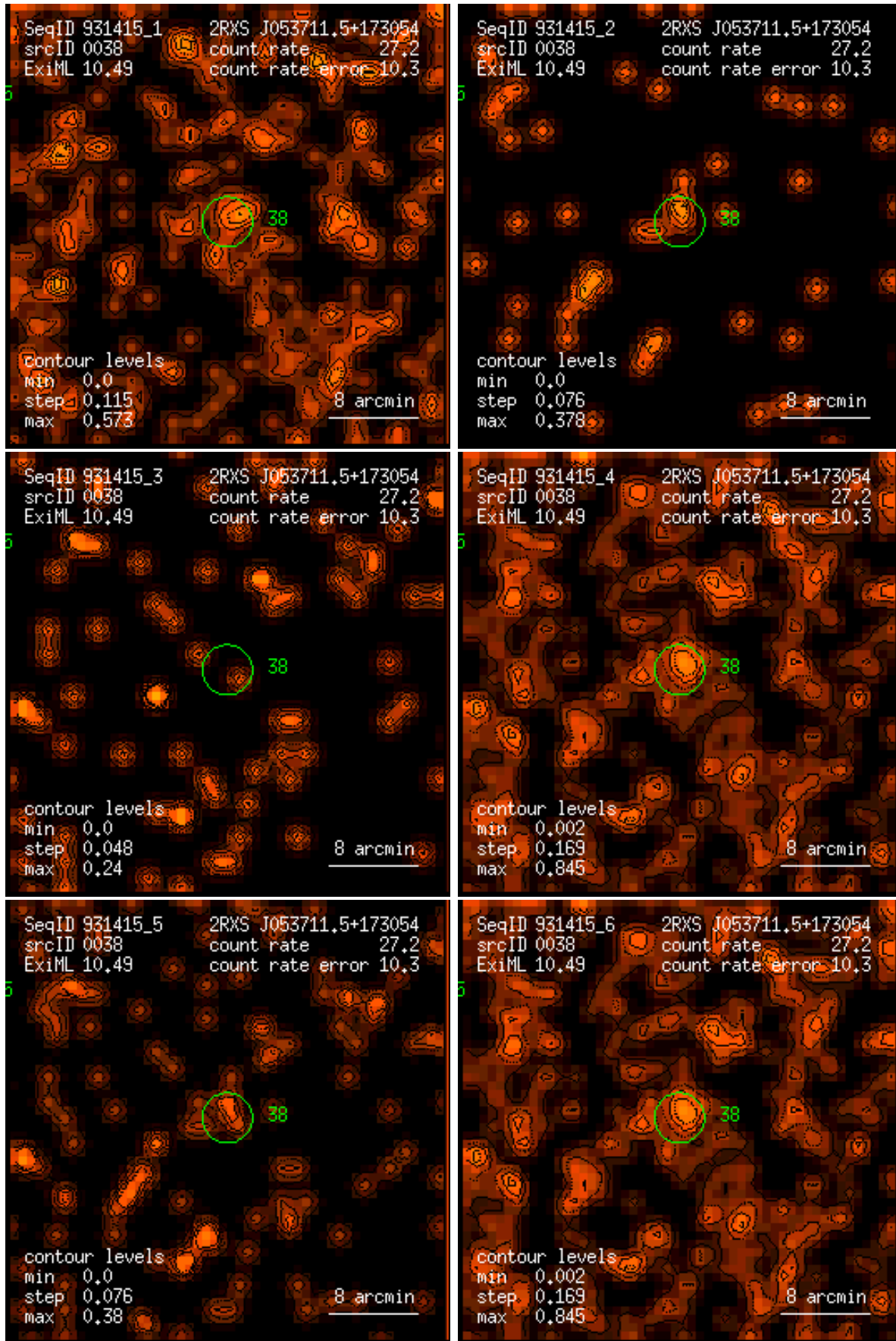
Figure 38: RASS 931415: detection 0038: band rate images, Gaussian filter: (1) PSPC channels 11 – 41, (2) 52 – 90, (3) 91 – 201, (4) 11 – 235, (5) 52 – 201, (6) 11 – 201. Broad band rates in counts/ks. Band rate contour levels in counts/ks/arcmin 2 .
