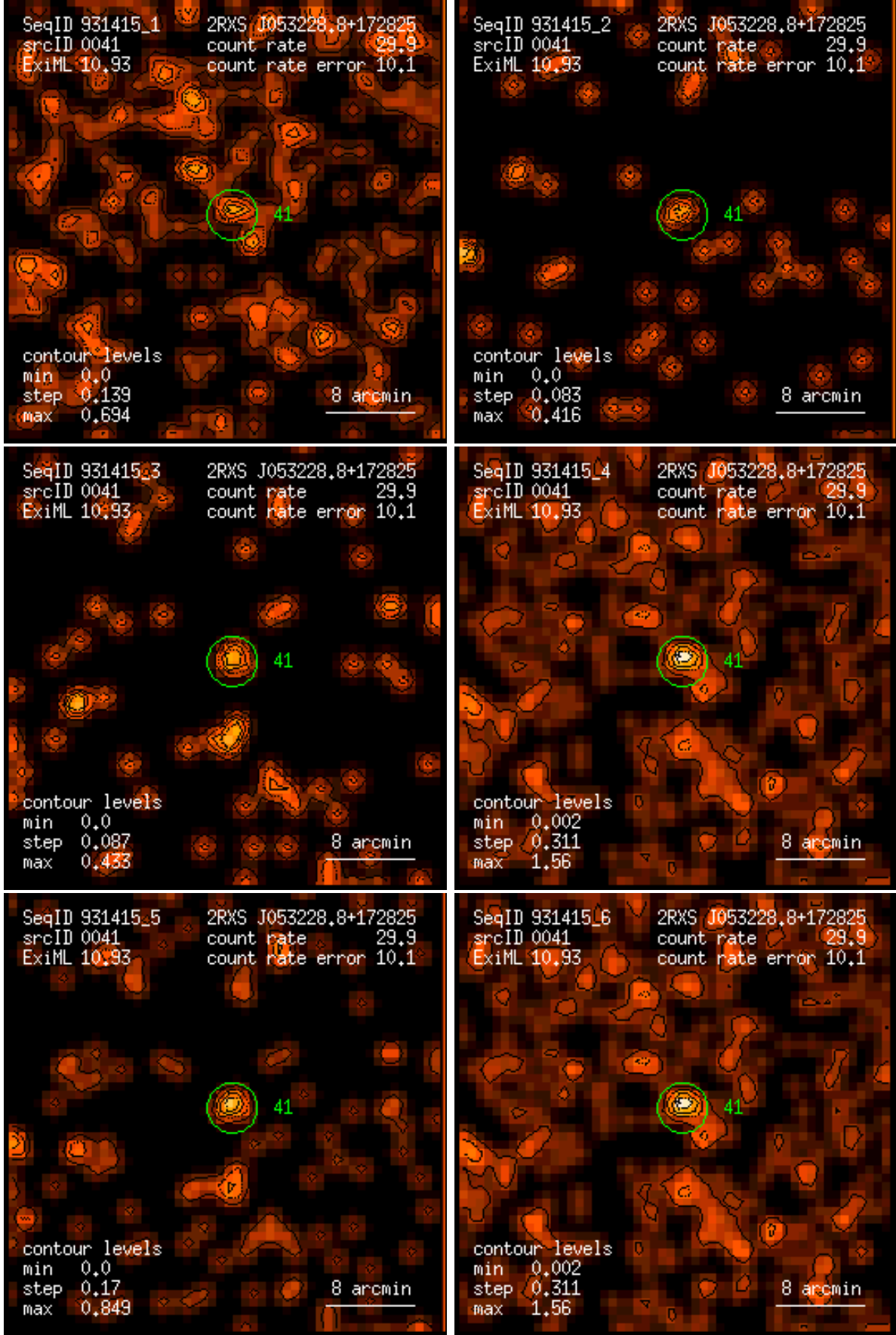
Figure 41: RASS 931415: detection 0041: band rate images, Gaussian filter: (1) PSPC channels 11 – 41, (2) 52 – 90, (3) 91 – 201, (4) 11 – 235, (5) 52 – 201, (6) 11 – 201. Broad band rates in counts/ks. Band rate contour levels in counts/ks/arcmin 2 .
