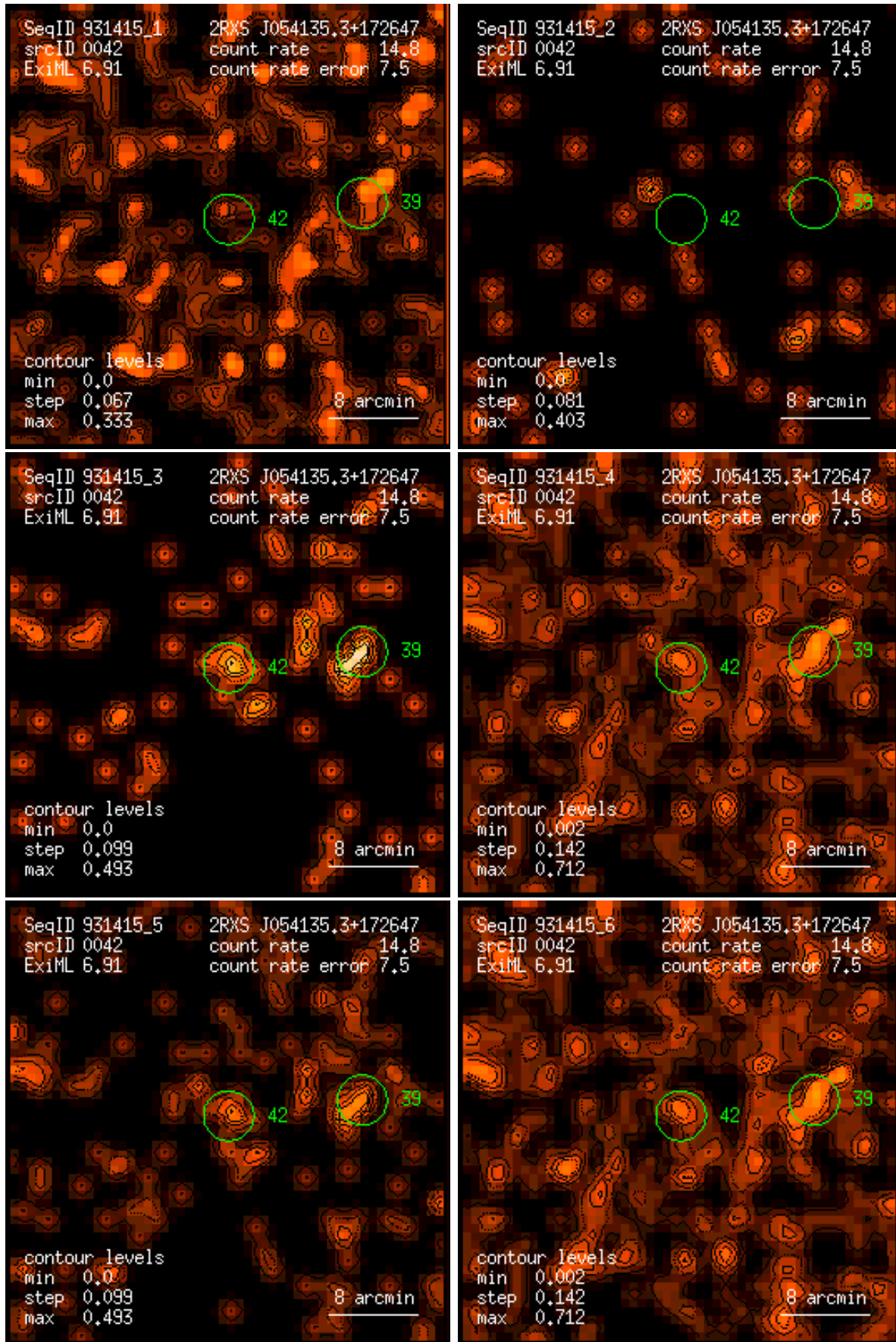
Figure 42: RASS 931415: detection 0042: band rate images, Gaussian filter: (1) PSPC channels 11 – 41, (2) 52 – 90, (3) 91 – 201, (4) 11 – 235, (5) 52 – 201, (6) 11 – 201. Broad band rates in counts/ks. Band rate contour levels in counts/ks/arcmin 2 .
