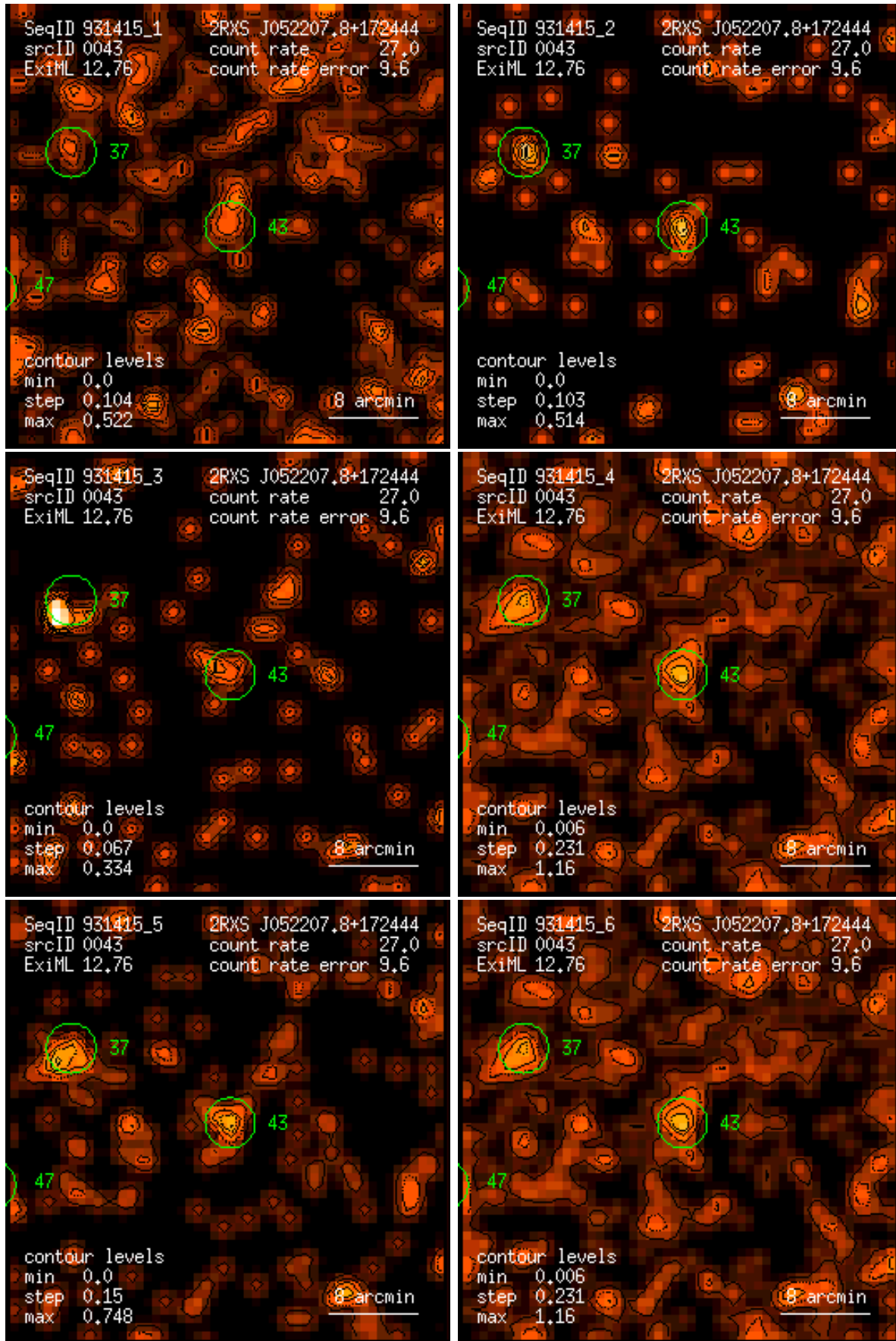
Figure 43: RASS 931415: detection 0043: band rate images, Gaussian filter: (1) PSPC channels 11 – 41, (2) 52 – 90, (3) 91 – 201, (4) 11 – 235, (5) 52 – 201, (6) 11 – 201. Broad band rates in counts/ks. Band rate contour levels in counts/ks/arcmin 2 .
