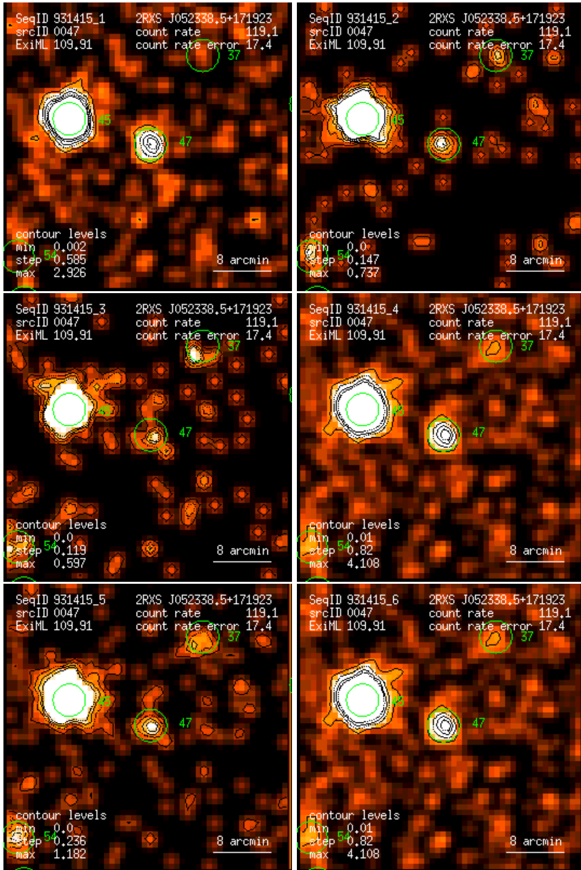
Figure 47: RASS 931415: detection 0047: band rate images, Gaussian filter: (1) PSPC channels 11 – 41, (2) 52 – 90, (3) 91 – 201, (4) 11 – 235, (5) 52 – 201, (6) 11 – 201. Broad band rates in counts/ks. Band rate contour levels in counts/ks/arcmin 2 .
