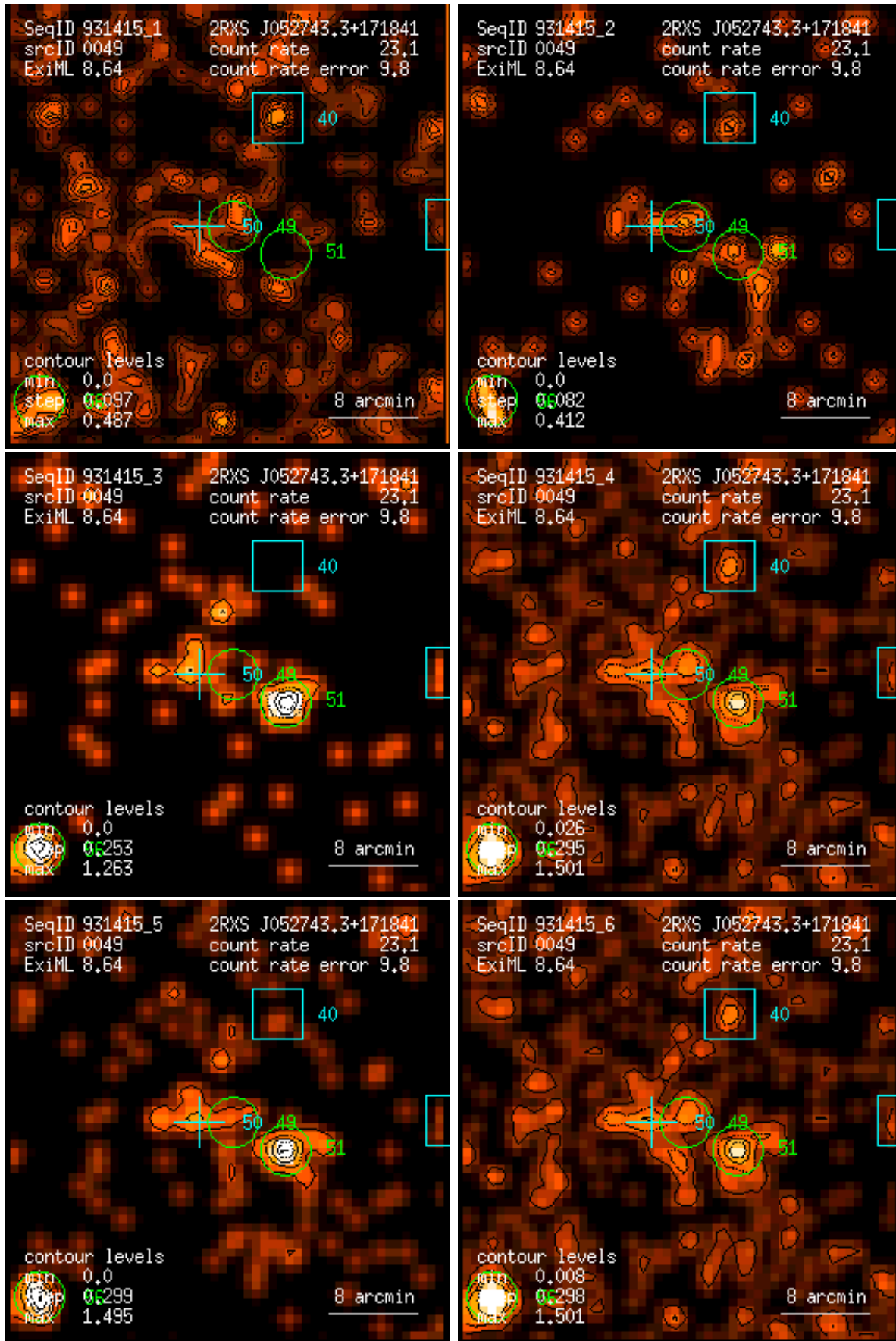
Figure 49: RASS 931415: detection 0049: band rate images, Gaussian filter: (1) PSPC channels 11 – 41, (2) 52 – 90, (3) 91 – 201, (4) 11 – 235, (5) 52 – 201, (6) 11 – 201. Broad band rates in counts/ks. Band rate contour levels in counts/ks/arcmin 2 .
