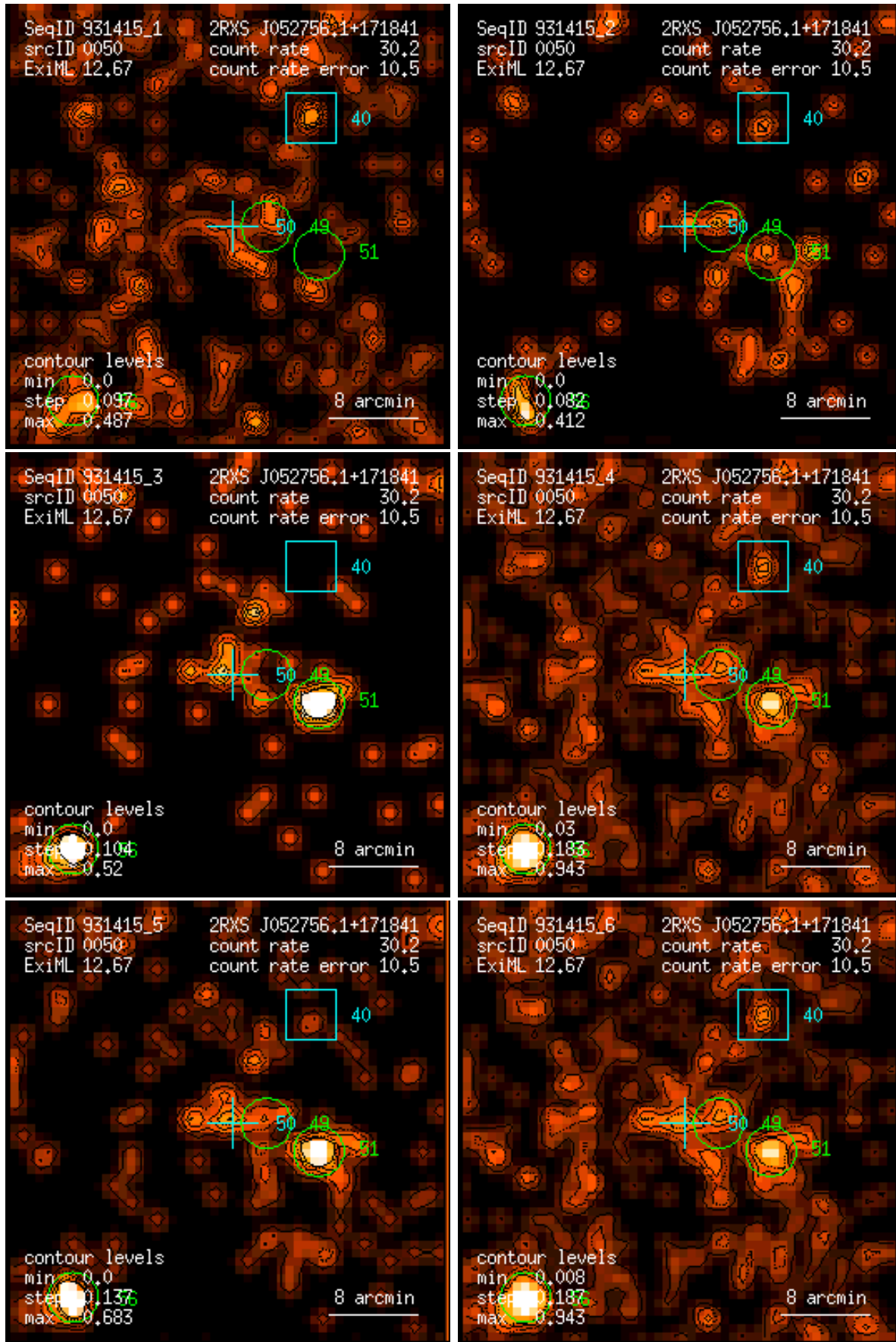
Figure 50: RASS 931415: detection 0050: band rate images, Gaussian filter: (1) PSPC channels 11 – 41, (2) 52 – 90, (3) 91 – 201, (4) 11 – 235, (5) 52 – 201, (6) 11 – 201. Broad band rates in counts/ks. Band rate contour levels in counts/ks/arcmin 2 .
