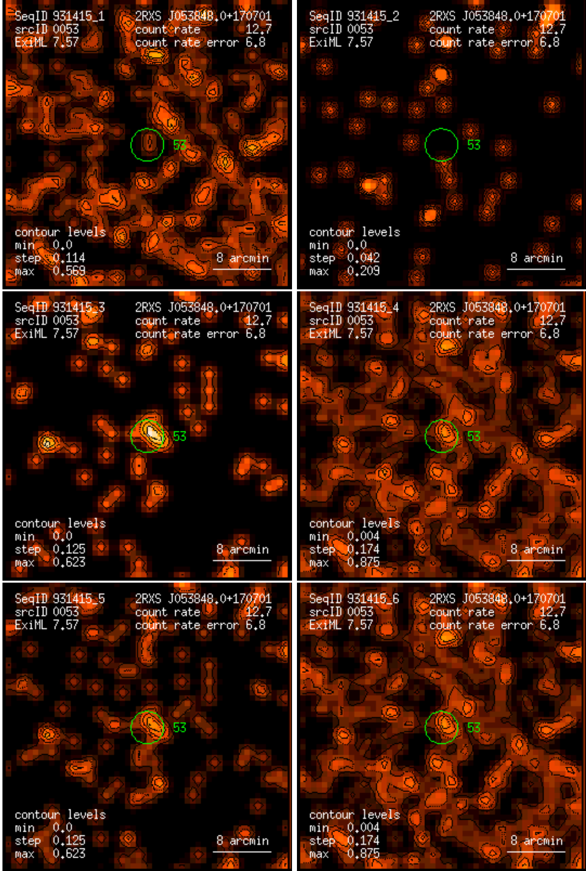
Figure 53: RASS 931415: detection 0053: band rate images, Gaussian filter: (1) PSPC channels 11 – 41, (2) 52 – 90, (3) 91 – 201, (4) 11 – 235, (5) 52 – 201, (6) 11 – 201. Broad band rates in counts/ks. Band rate contour levels in counts/ks/arcmin 2 .
