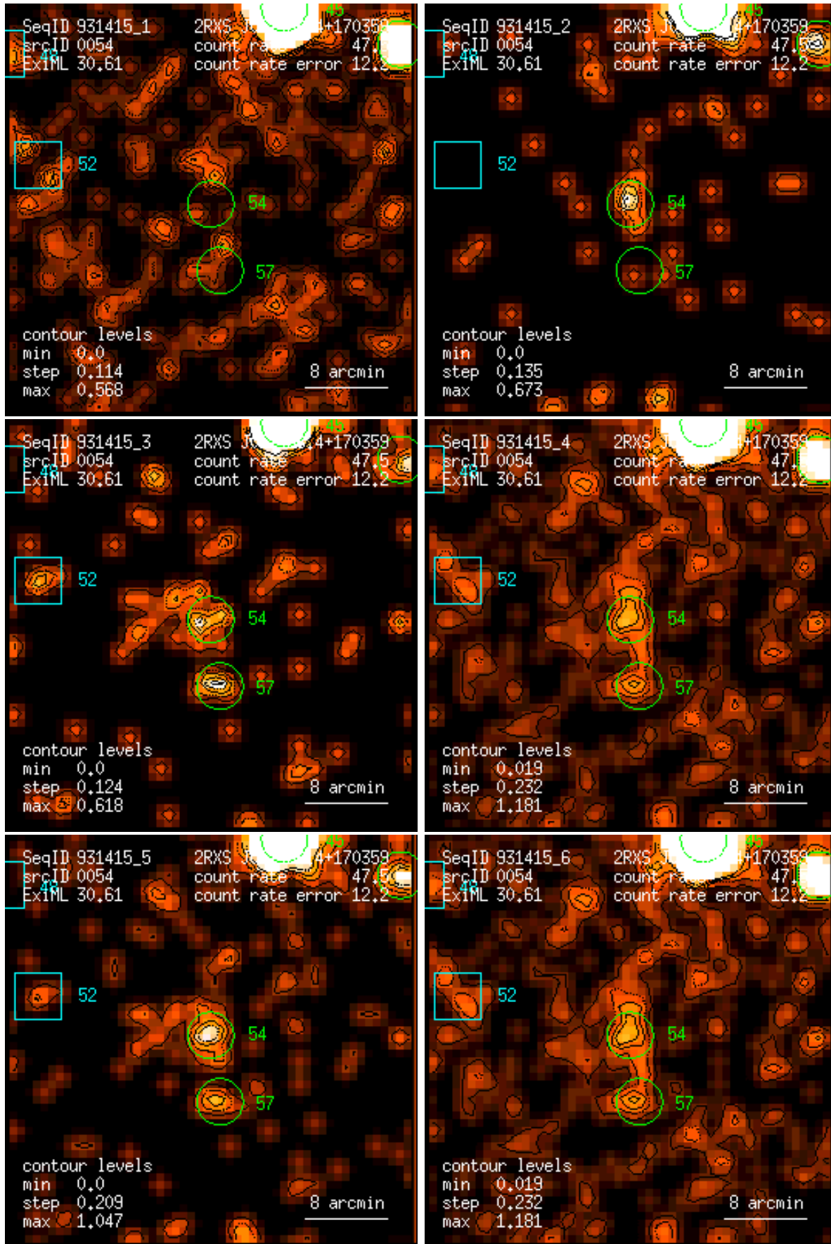
Figure 54: RASS 931415: detection 0054: band rate images, Gaussian filter: (1) PSPC channels 11 – 41, (2) 52 – 90, (3) 91 – 201, (4) 11 – 235, (5) 52 – 201, (6) 11 – 201. Broad band rates in counts/ks. Band rate contour levels in counts/ks/arcmin 2 .
