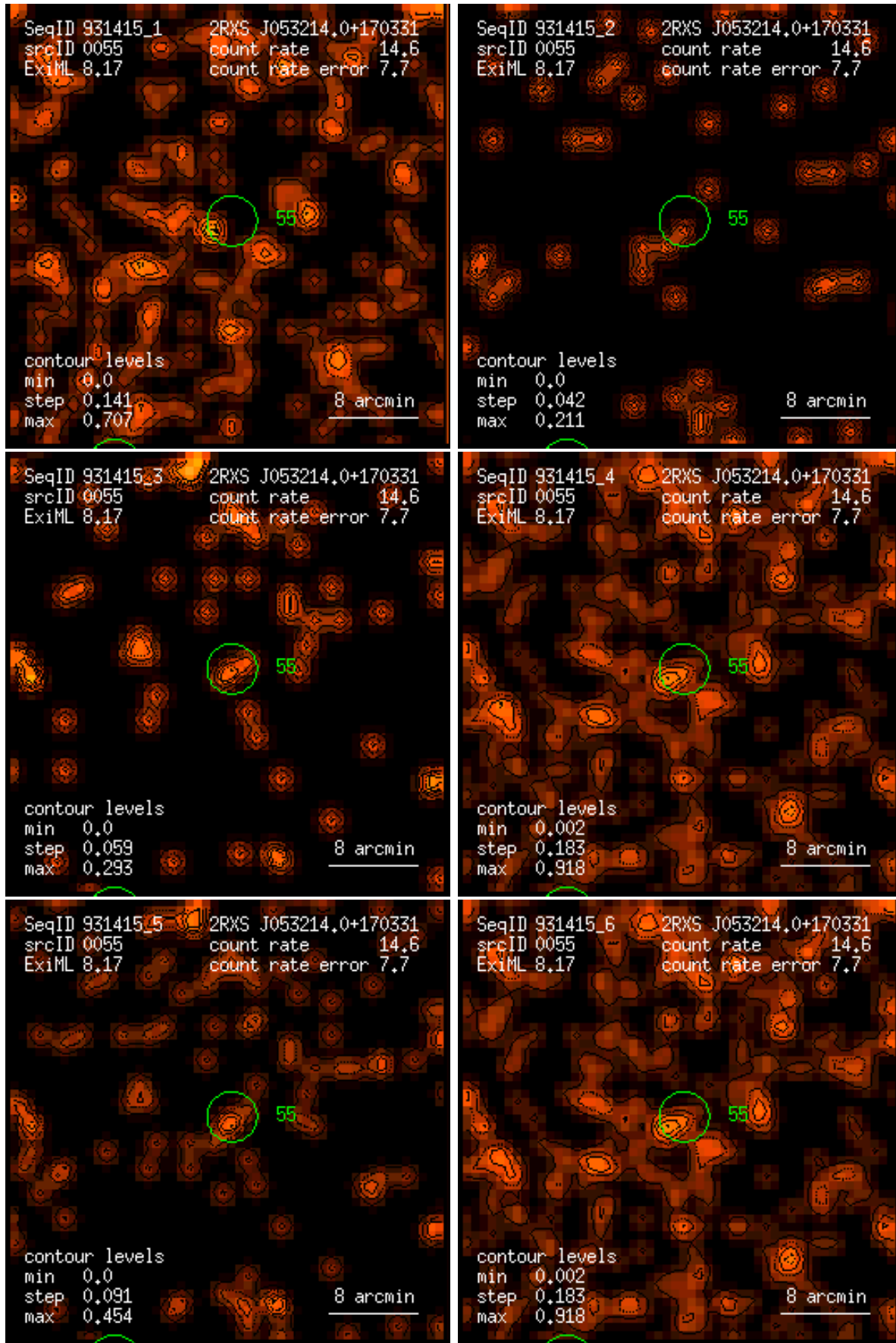
Figure 55: RASS 931415: detection 0055: band rate images, Gaussian filter: (1) PSPC channels 11 – 41, (2) 52 – 90, (3) 91 – 201, (4) 11 – 235, (5) 52 – 201, (6) 11 – 201. Broad band rates in counts/ks. Band rate contour levels in counts/ks/arcmin 2 .
