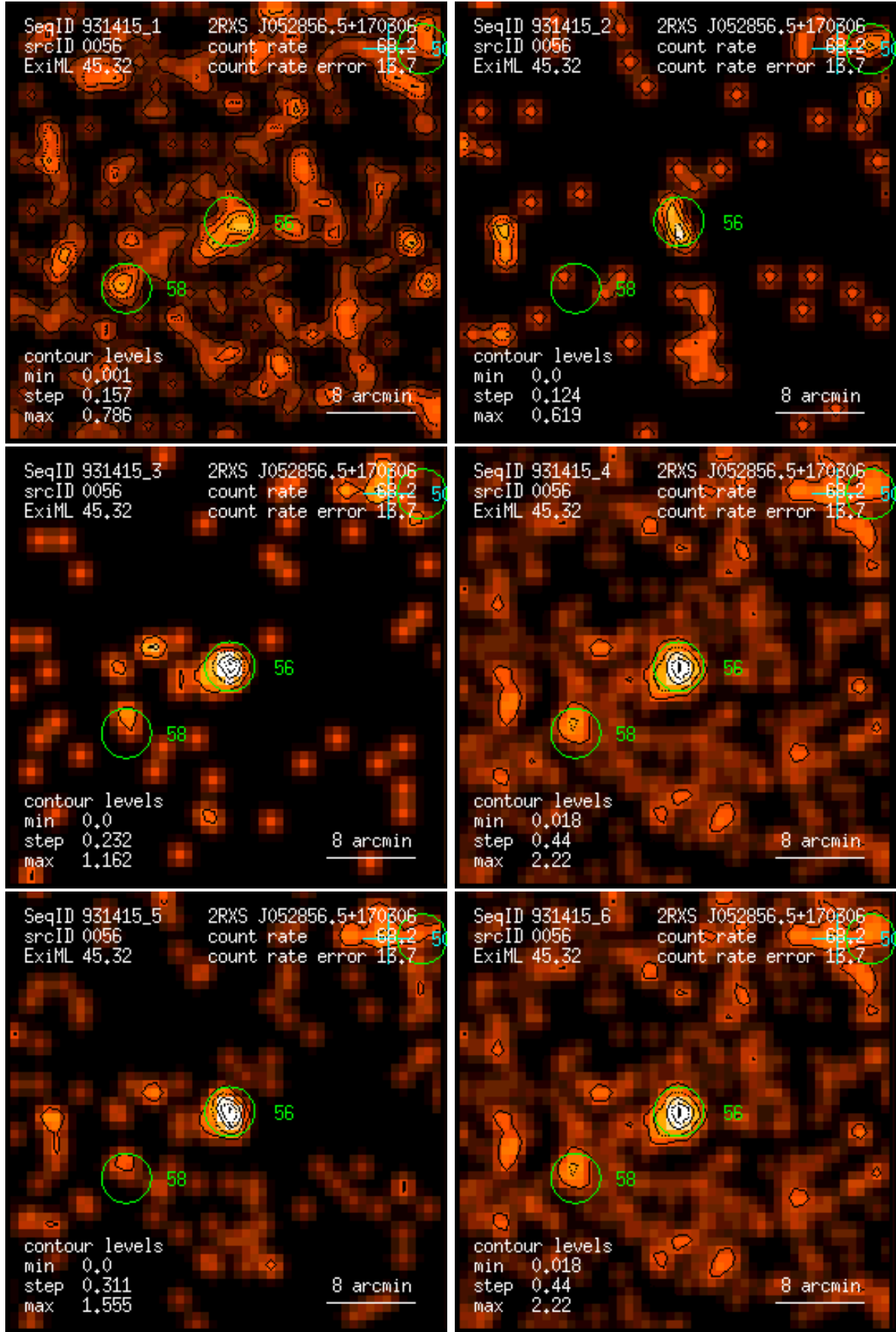
Figure 56: RASS 931415: detection 0056: band rate images, Gaussian filter: (1) PSPC channels 11 – 41, (2) 52 – 90, (3) 91 – 201, (4) 11 – 235, (5) 52 – 201, (6) 11 – 201. Broad band rates in counts/ks. Band rate contour levels in counts/ks/arcmin 2 .
