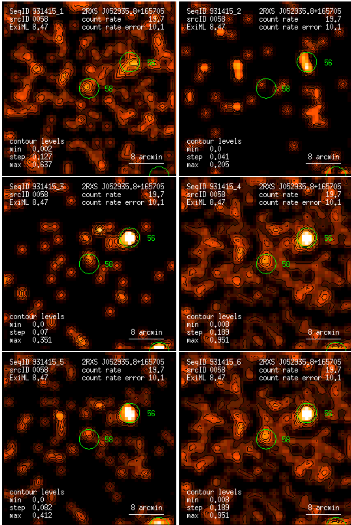
Figure 58: RASS 931415: detection 0058: band rate images, Gaussian filter: (1) PSPC channels 11 – 41, (2) 52 – 90, (3) 91 – 201, (4) 11 – 235, (5) 52 – 201, (6) 11 – 201. Broad band rates in counts/ks. Band rate contour levels in counts/ks/arcmin 2 .
