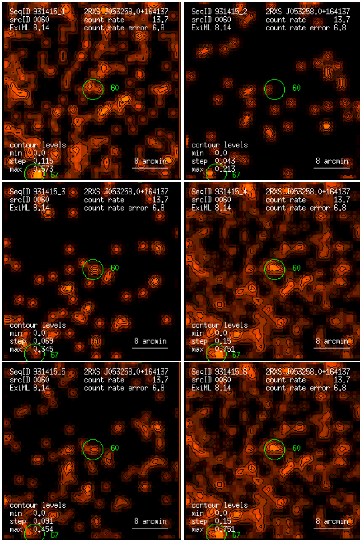
Figure 60: RASS 931415: detection 0060: band rate images, Gaussian filter: (1) PSPC channels 11 – 41, (2) 52 – 90, (3) 91 – 201, (4) 11 – 235, (5) 52 – 201, (6) 11 – 201. Broad band rates in counts/ks. Band rate contour levels in counts/ks/arcmin 2 .
