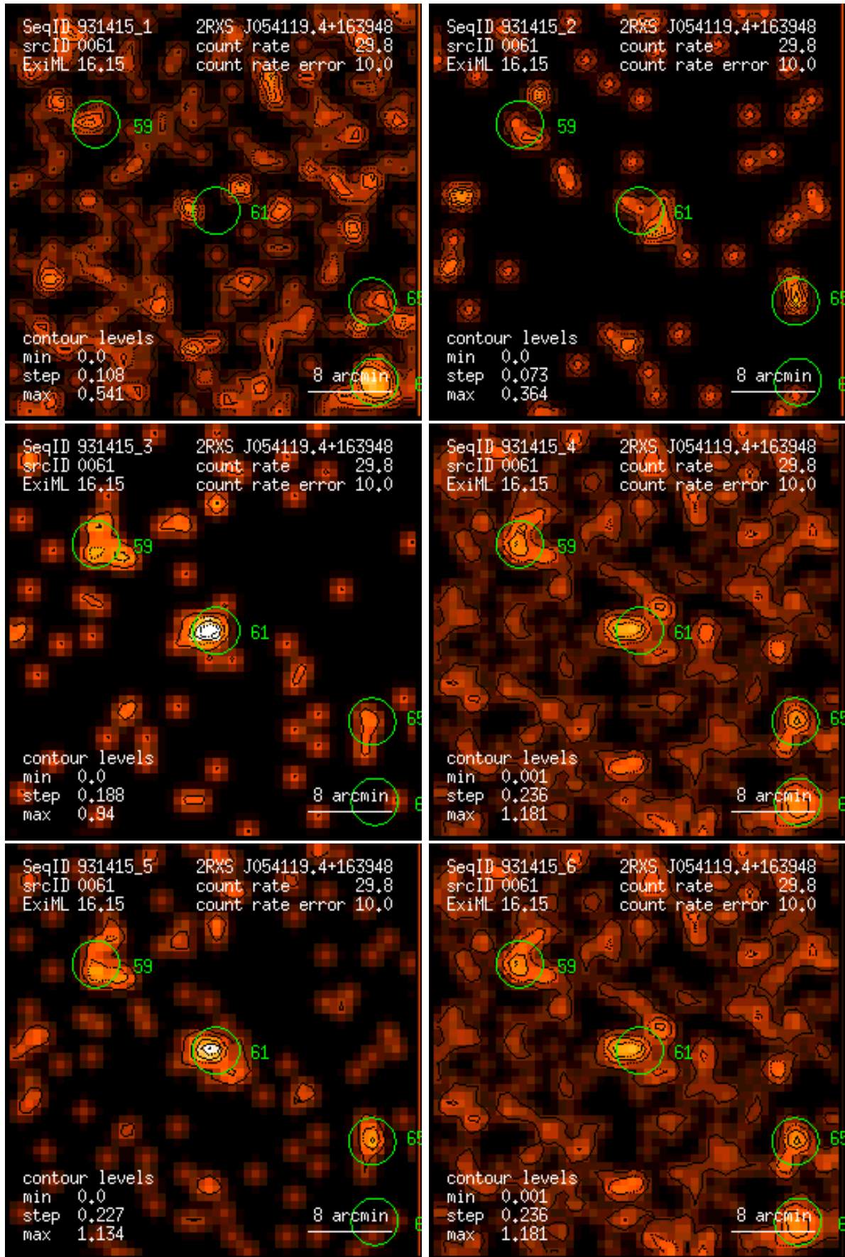
Figure 61: RASS 931415: detection 0061: band rate images, Gaussian filter: (1) PSPC channels 11 – 41, (2) 52 – 90, (3) 91 – 201, (4) 11 – 235, (5) 52 – 201, (6) 11 – 201. Broad band rates in counts/ks. Band rate contour levels in counts/ks/arcmin 2 .
