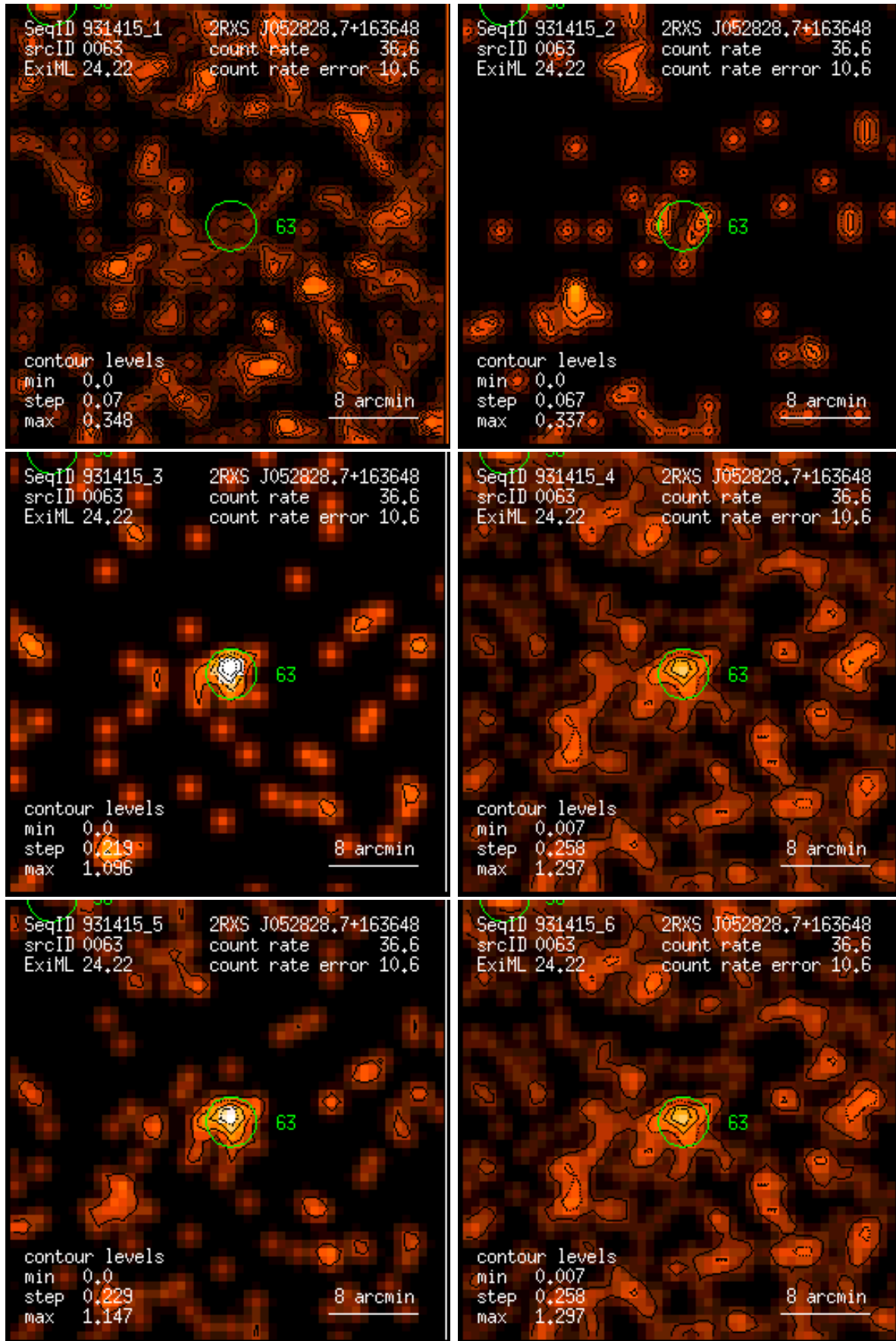
Figure 63: RASS 931415: detection 0063: band rate images, Gaussian filter: (1) PSPC channels 11 – 41, (2) 52 – 90, (3) 91 – 201, (4) 11 – 235, (5) 52 – 201, (6) 11 – 201. Broad band rates in counts/ks. Band rate contour levels in counts/ks/arcmin 2 .
