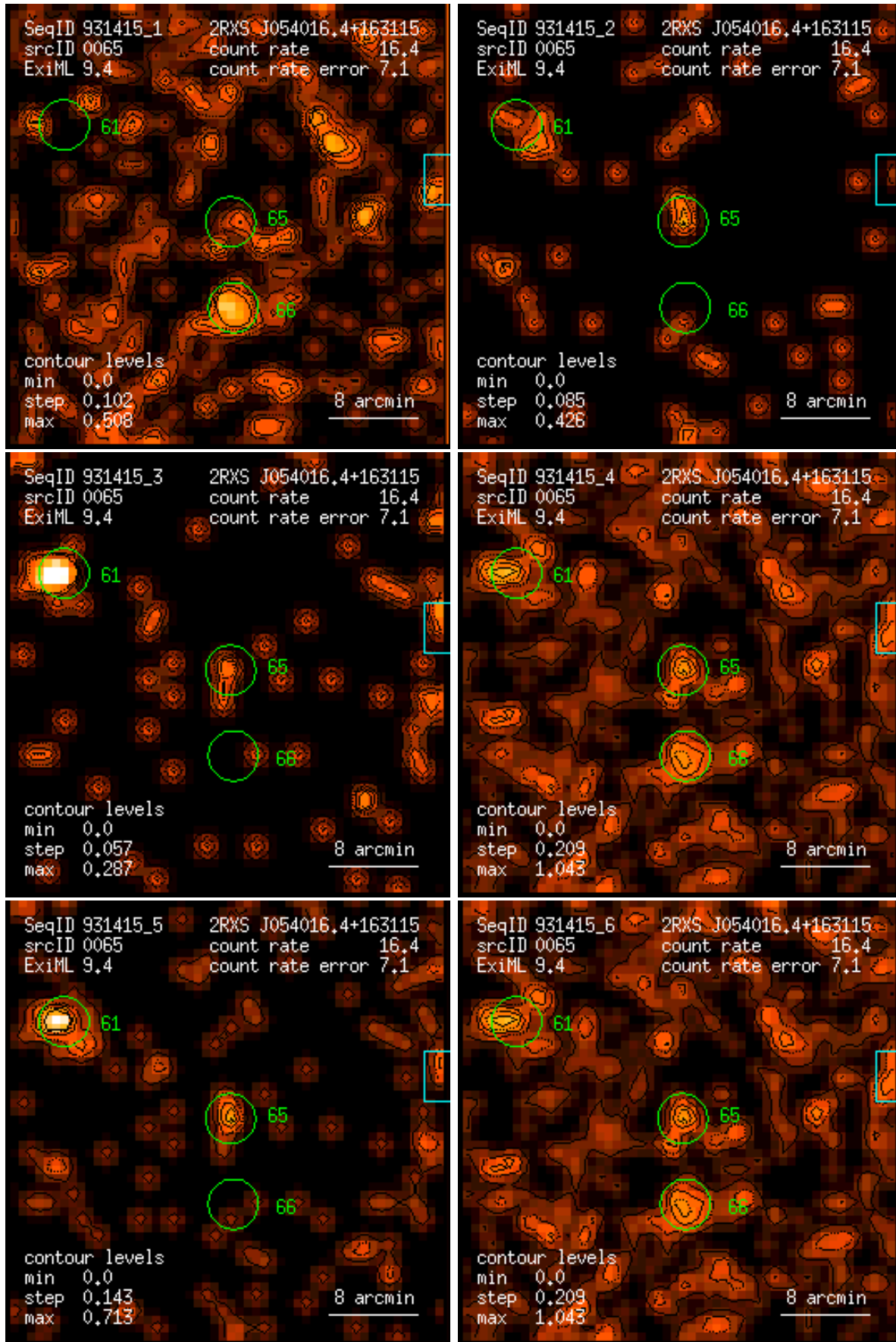
Figure 65: RASS 931415: detection 0065: band rate images, Gaussian filter: (1) PSPC channels 11 – 41, (2) 52 – 90, (3) 91 – 201, (4) 11 – 235, (5) 52 – 201, (6) 11 – 201. Broad band rates in counts/ks. Band rate contour levels in counts/ks/arcmin 2 .
