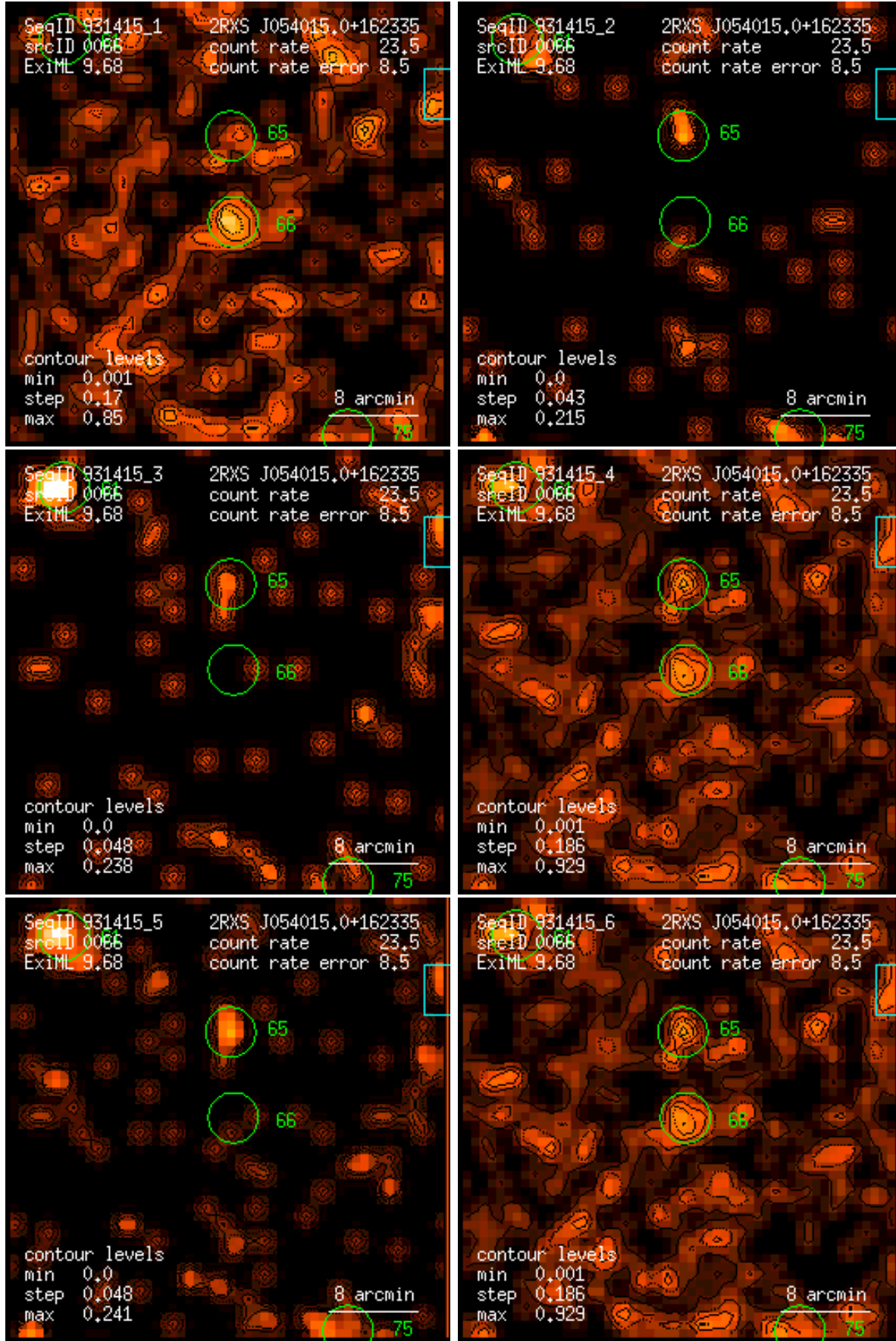
Figure 66: RASS 931415: detection 0066: band rate images, Gaussian filter: (1) PSPC channels 11 – 41, (2) 52 – 90, (3) 91 – 201, (4) 11 – 235, (5) 52 – 201, (6) 11 – 201. Broad band rates in counts/ks. Band rate contour levels in counts/ks/arcmin 2 .
