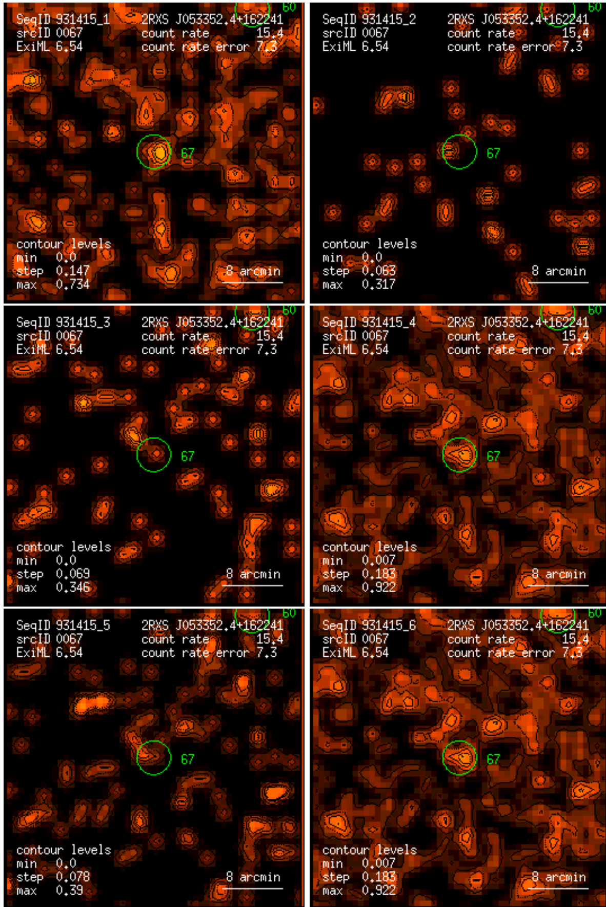
Figure 67: RASS 931415: detection 0067: band rate images, Gaussian filter: (1) PSPC channels 11 – 41, (2) 52 – 90, (3) 91 – 201, (4) 11 – 235, (5) 52 – 201, (6) 11 – 201. Broad band rates in counts/ks. Band rate contour levels in counts/ks/arcmin 2 .
