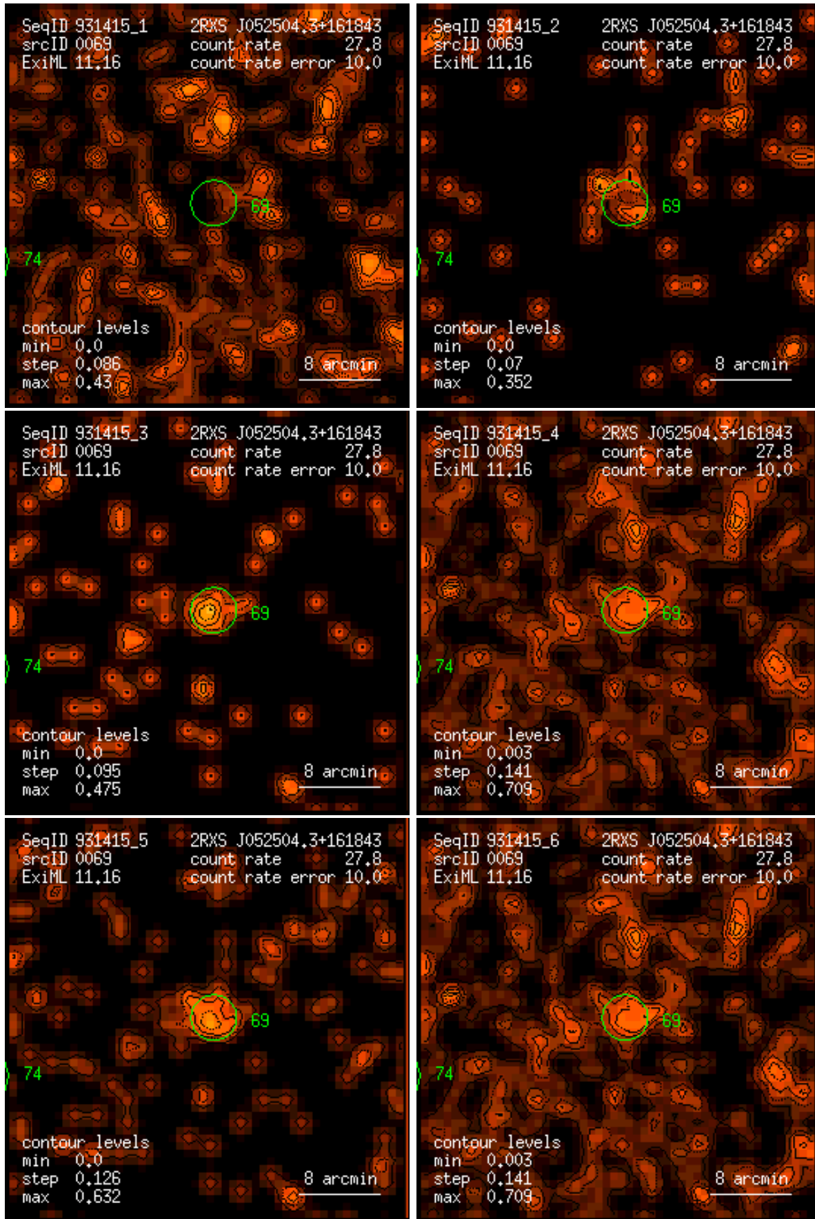
Figure 69: RASS 931415: detection 0069: band rate images, Gaussian filter: (1) PSPC channels 11 – 41, (2) 52 – 90, (3) 91 – 201, (4) 11 – 235, (5) 52 – 201, (6) 11 – 201. Broad band rates in counts/ks. Band rate contour levels in counts/ks/arcmin 2 .
