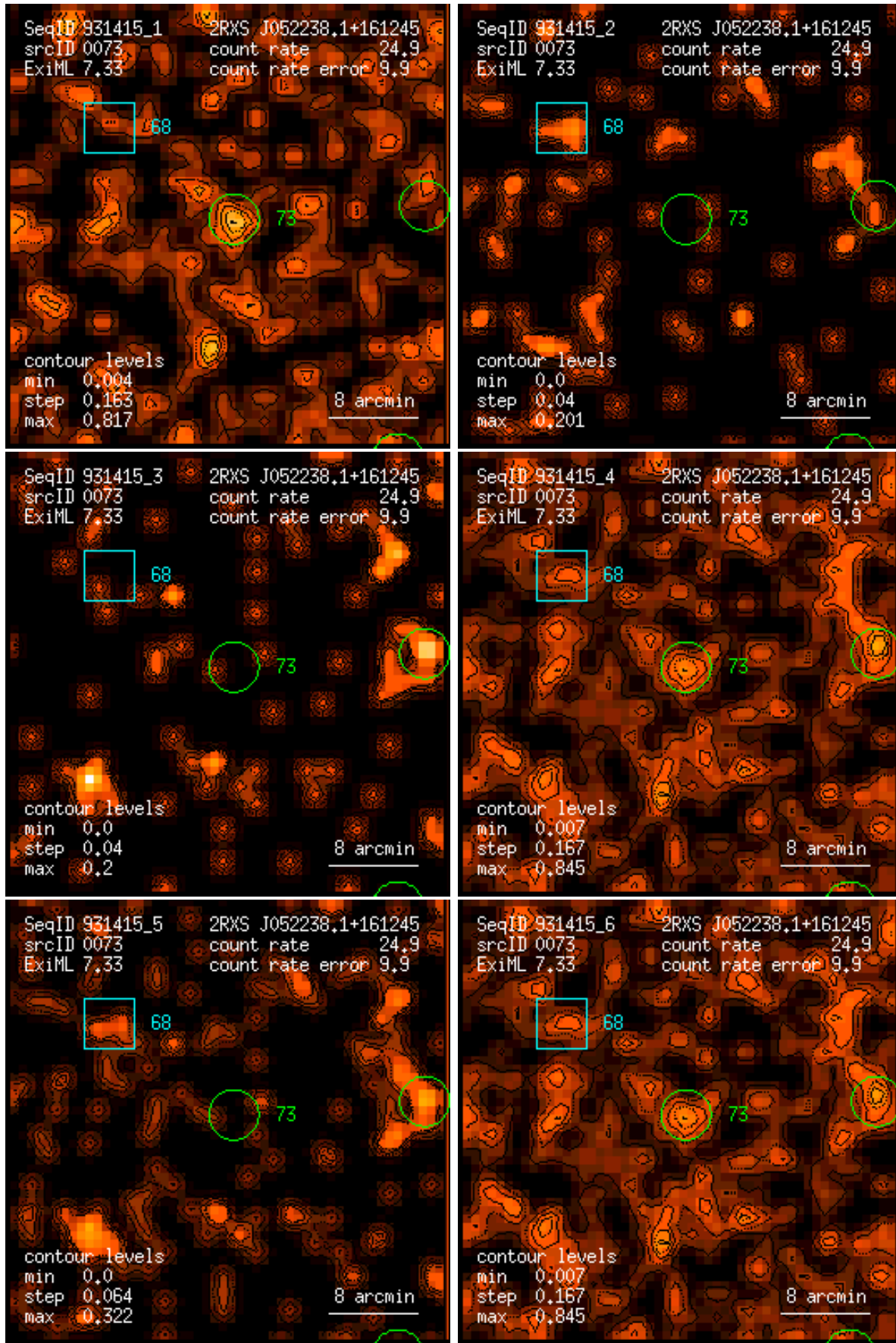
Figure 73: RASS 931415: detection 0073: band rate images, Gaussian filter: (1) PSPC channels 11 – 41, (2) 52 – 90, (3) 91 – 201, (4) 11 – 235, (5) 52 – 201, (6) 11 – 201. Broad band rates in counts/ks. Band rate contour levels in counts/ks/arcmin 2 .
