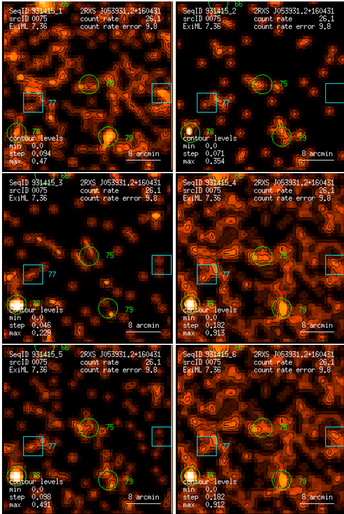
Figure 75: RASS 931415: detection 0075: band rate images, Gaussian filter: (1) PSPC channels 11 – 41, (2) 52 – 90, (3) 91 – 201, (4) 11 – 235, (5) 52 – 201, (6) 11 – 201. Broad band rates in counts/ks. Band rate contour levels in counts/ks/arcmin 2 .
