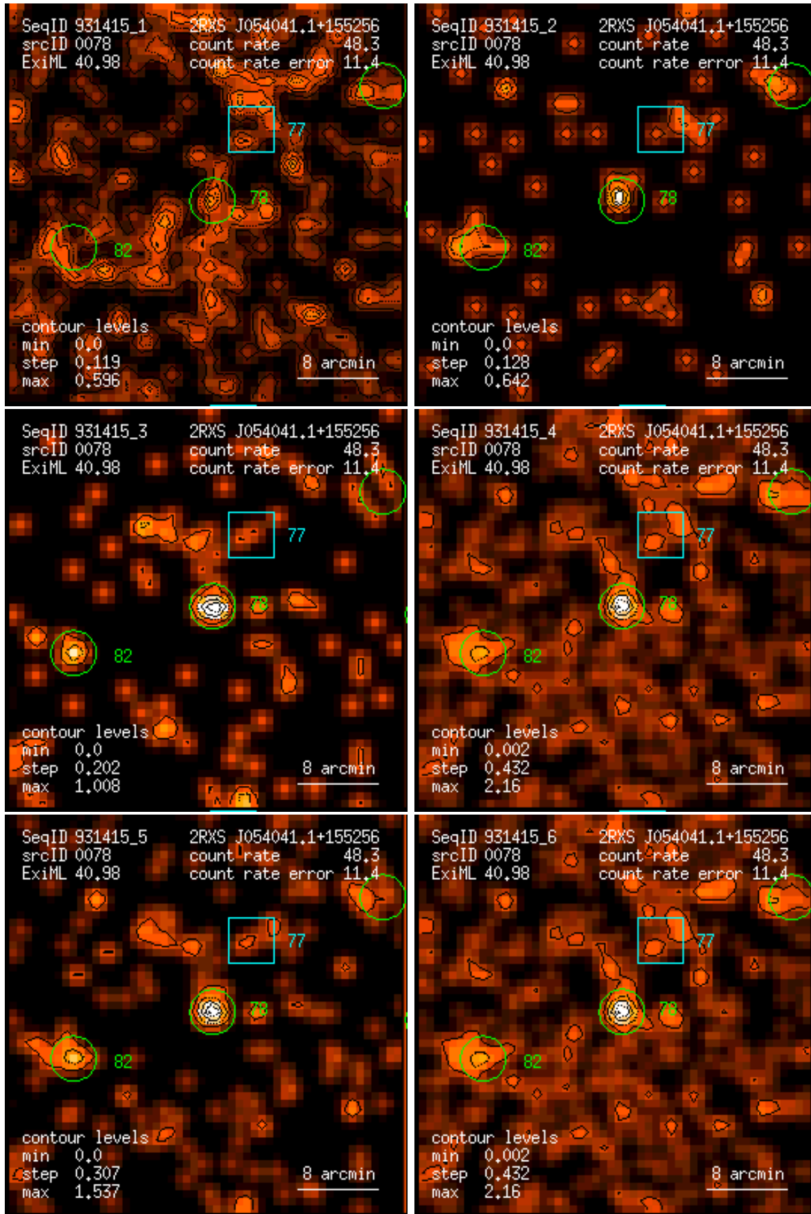
Figure 78: RASS 931415: detection 0078: band rate images, Gaussian filter: (1) PSPC channels 11 – 41, (2) 52 – 90, (3) 91 – 201, (4) 11 – 235, (5) 52 – 201, (6) 11 – 201. Broad band rates in counts/ks. Band rate contour levels in counts/ks/arcmin 2 .
