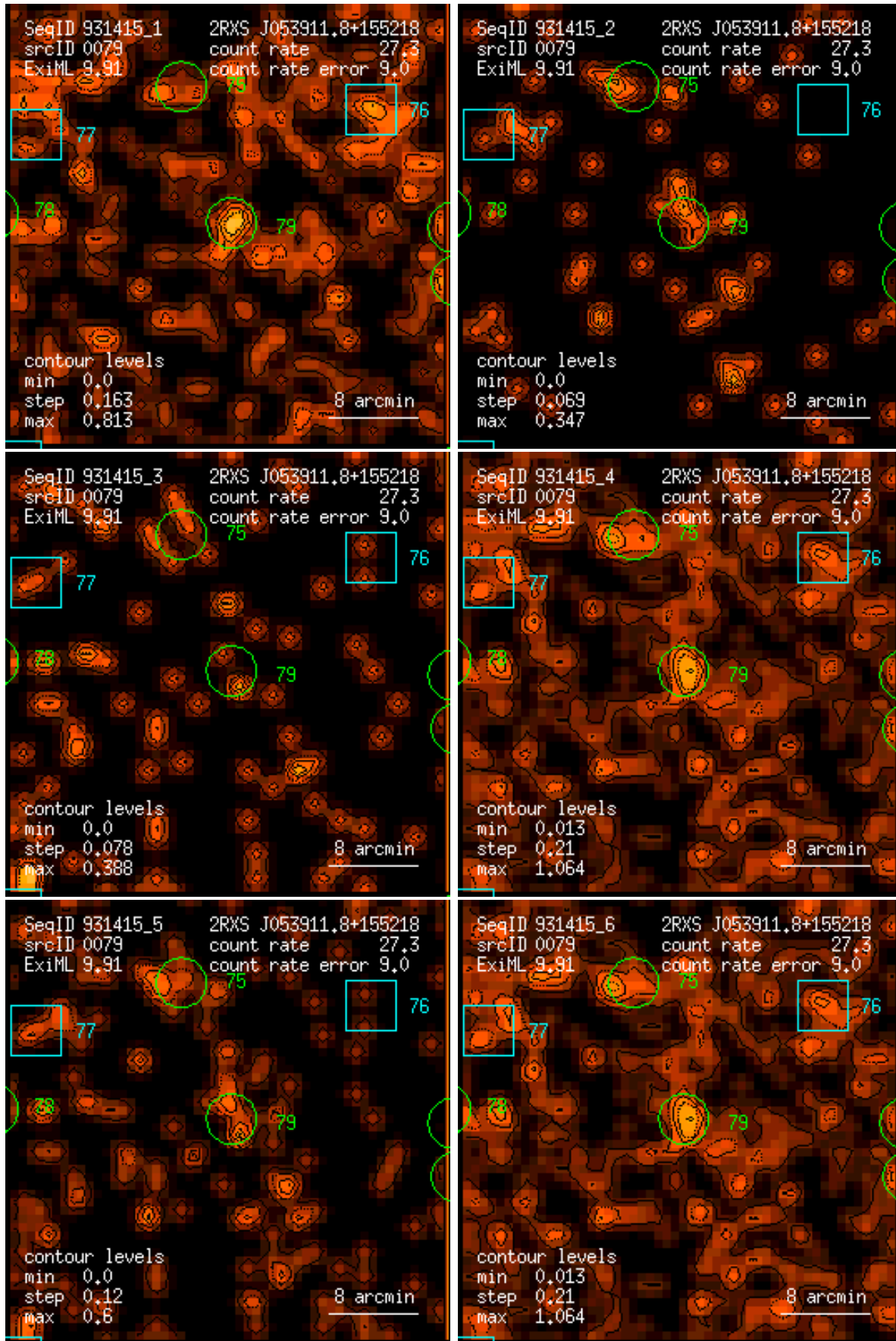
Figure 79: RASS 931415: detection 0079: band rate images, Gaussian filter: (1) PSPC channels 11 – 41, (2) 52 – 90, (3) 91 – 201, (4) 11 – 235, (5) 52 – 201, (6) 11 – 201. Broad band rates in counts/ks. Band rate contour levels in counts/ks/arcmin 2 .
