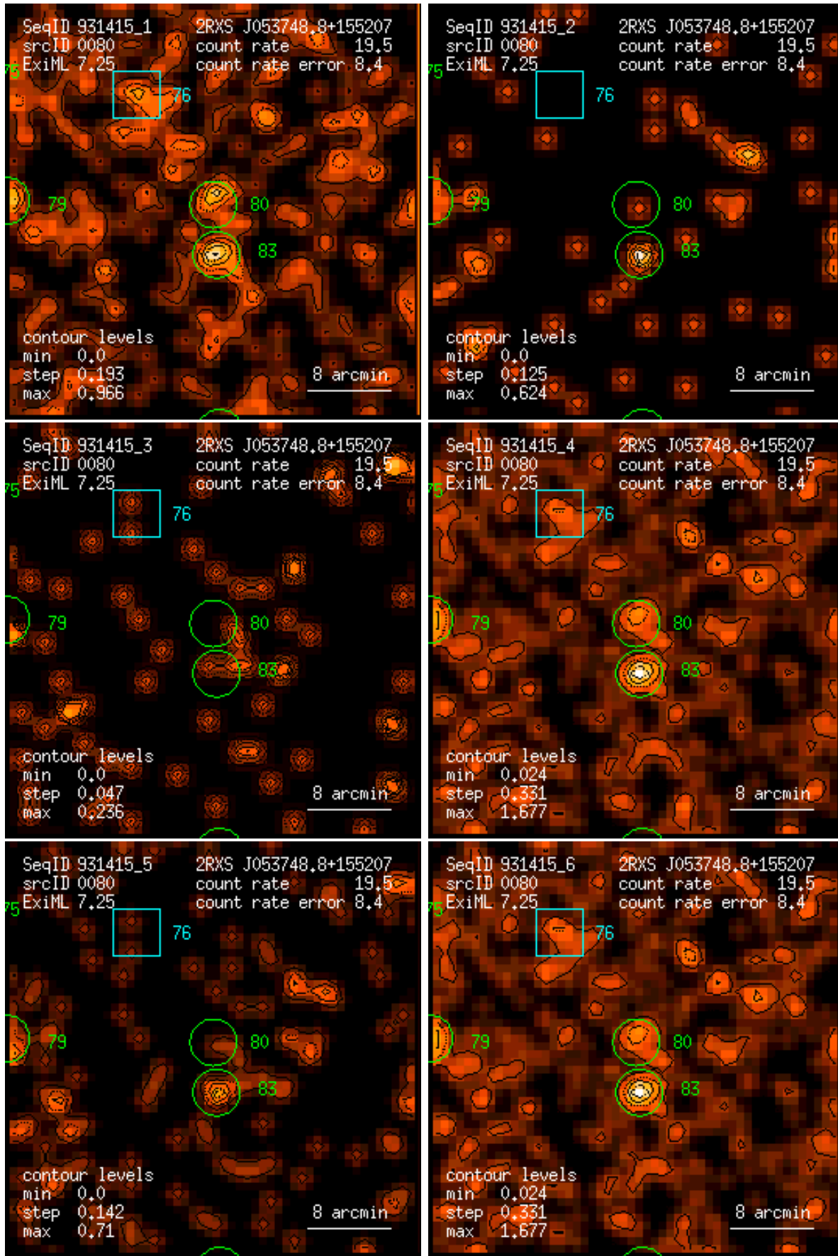
Figure 80: RASS 931415: detection 0080: band rate images, Gaussian filter: (1) PSPC channels 11 – 41, (2) 52 – 90, (3) 91 – 201, (4) 11 – 235, (5) 52 – 201, (6) 11 – 201. Broad band rates in counts/ks. Band rate contour levels in counts/ks/arcmin 2 .
