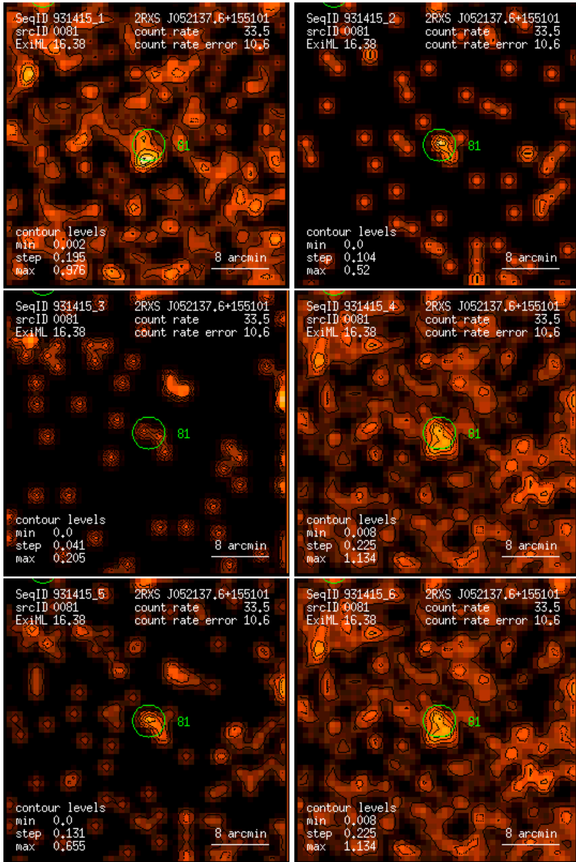
Figure 81: RASS 931415: detection 0081: band rate images, Gaussian filter: (1) PSPC channels 11 – 41, (2) 52 – 90, (3) 91 – 201, (4) 11 – 235, (5) 52 – 201, (6) 11 – 201. Broad band rates in counts/ks. Band rate contour levels in counts/ks/arcmin 2 .
