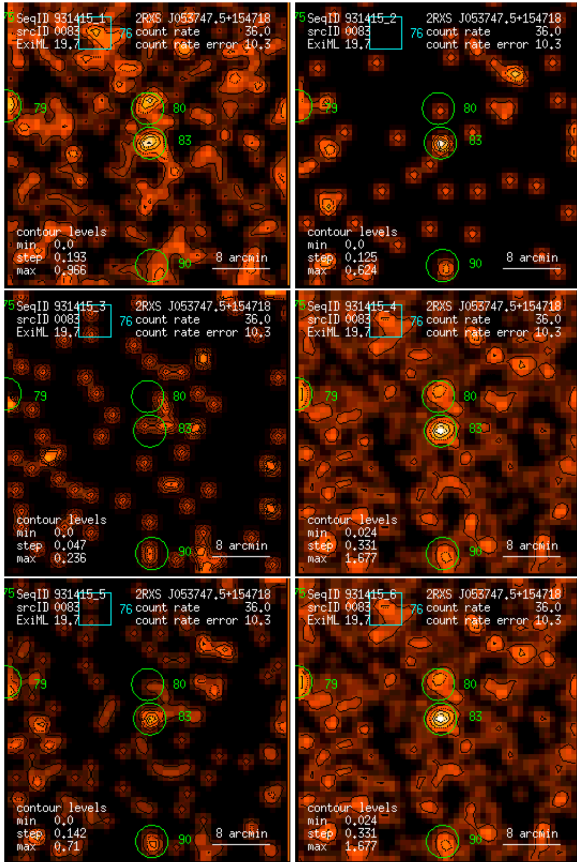
Figure 83: RASS 931415: detection 0083: band rate images, Gaussian filter: (1) PSPC channels 11 – 41, (2) 52 – 90, (3) 91 – 201, (4) 11 – 235, (5) 52 – 201, (6) 11 – 201. Broad band rates in counts/ks. Band rate contour levels in counts/ks/arcmin 2 .
