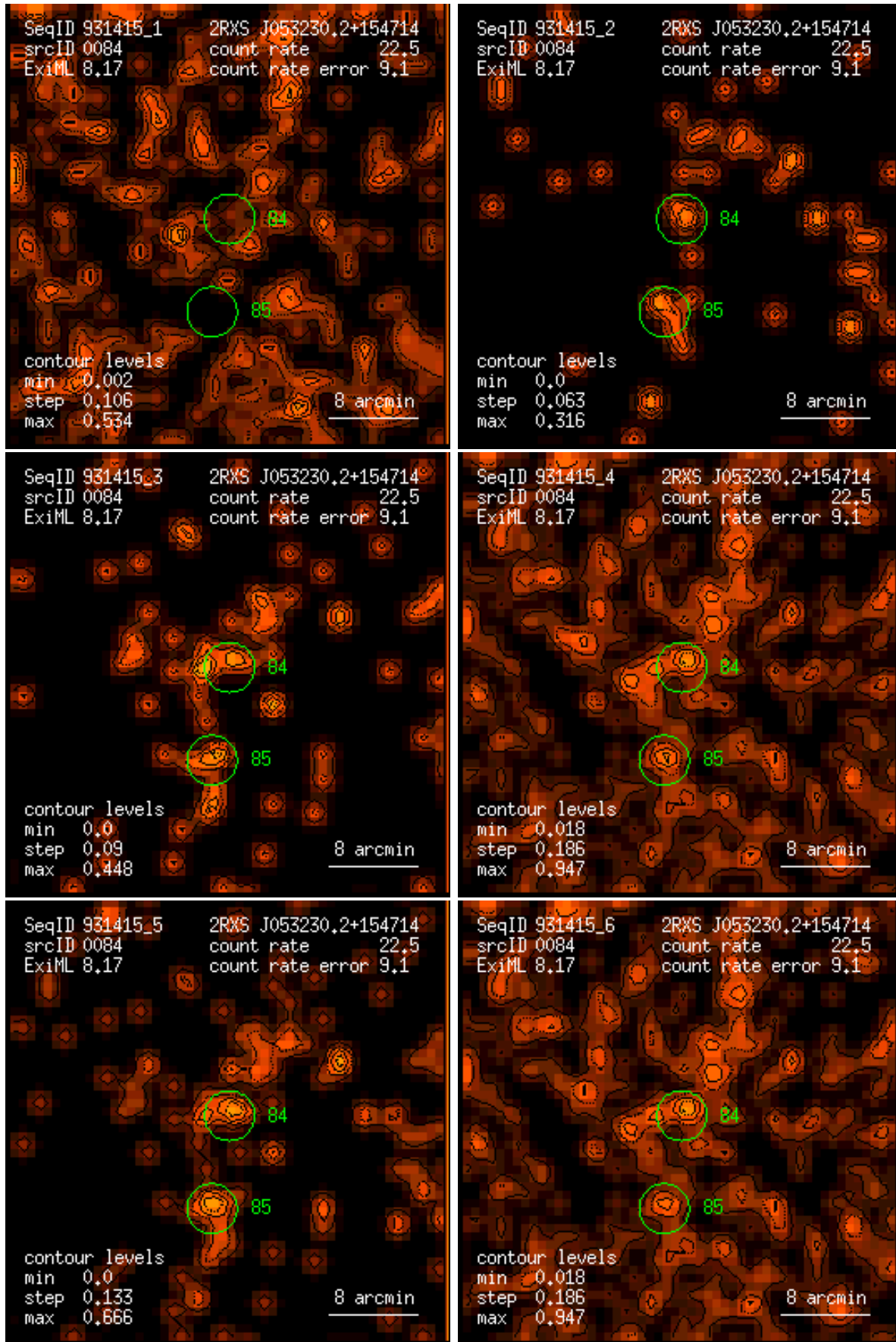
Figure 84: RASS 931415: detection 0084: band rate images, Gaussian filter: (1) PSPC channels 11 – 41, (2) 52 – 90, (3) 91 – 201, (4) 11 – 235, (5) 52 – 201, (6) 11 – 201. Broad band rates in counts/ks. Band rate contour levels in counts/ks/arcmin 2 .
