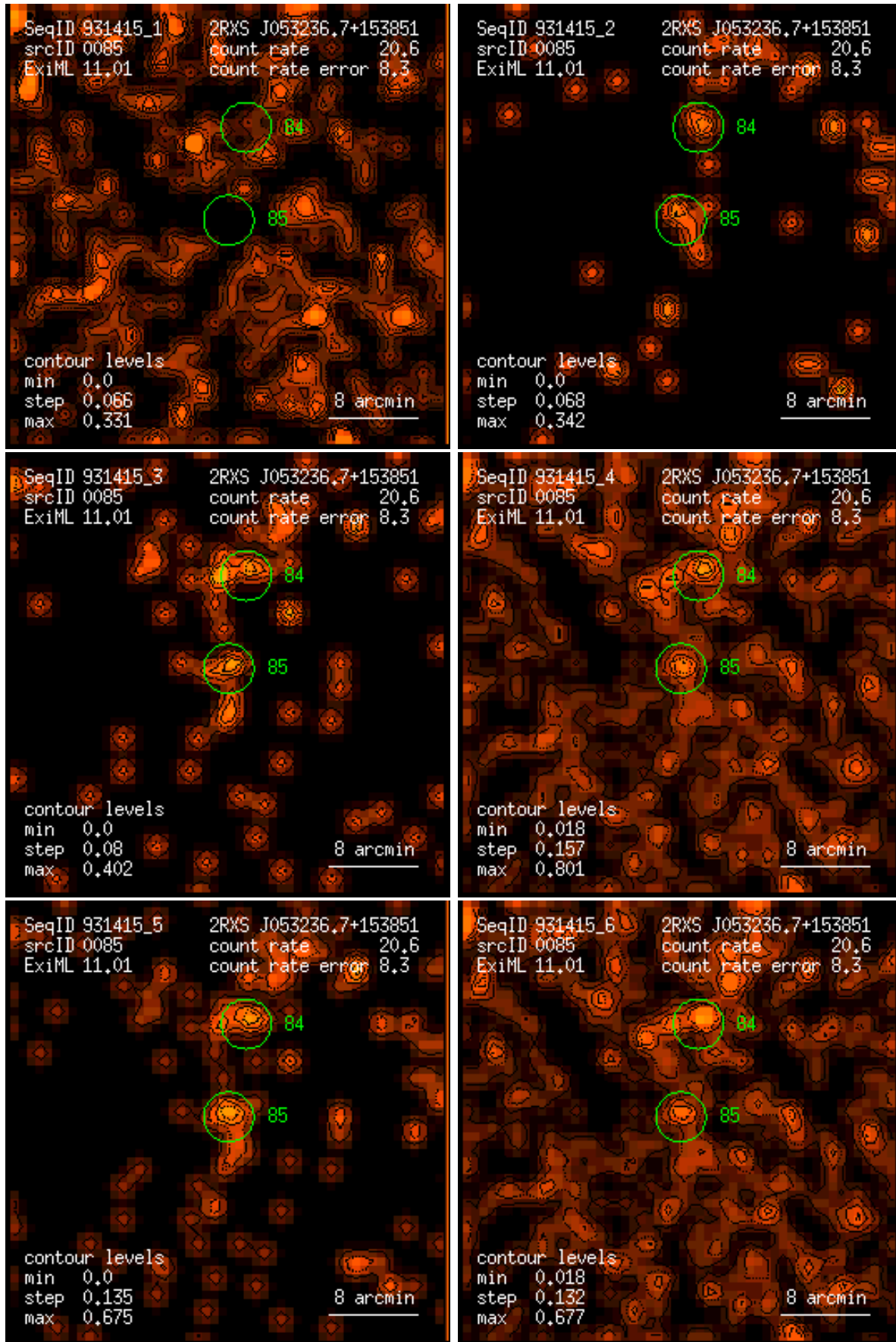
Figure 85: RASS 931415: detection 0085: band rate images, Gaussian filter: (1) PSPC channels 11 – 41, (2) 52 – 90, (3) 91 – 201, (4) 11 – 235, (5) 52 – 201, (6) 11 – 201. Broad band rates in counts/ks. Band rate contour levels in counts/ks/arcmin 2 .
