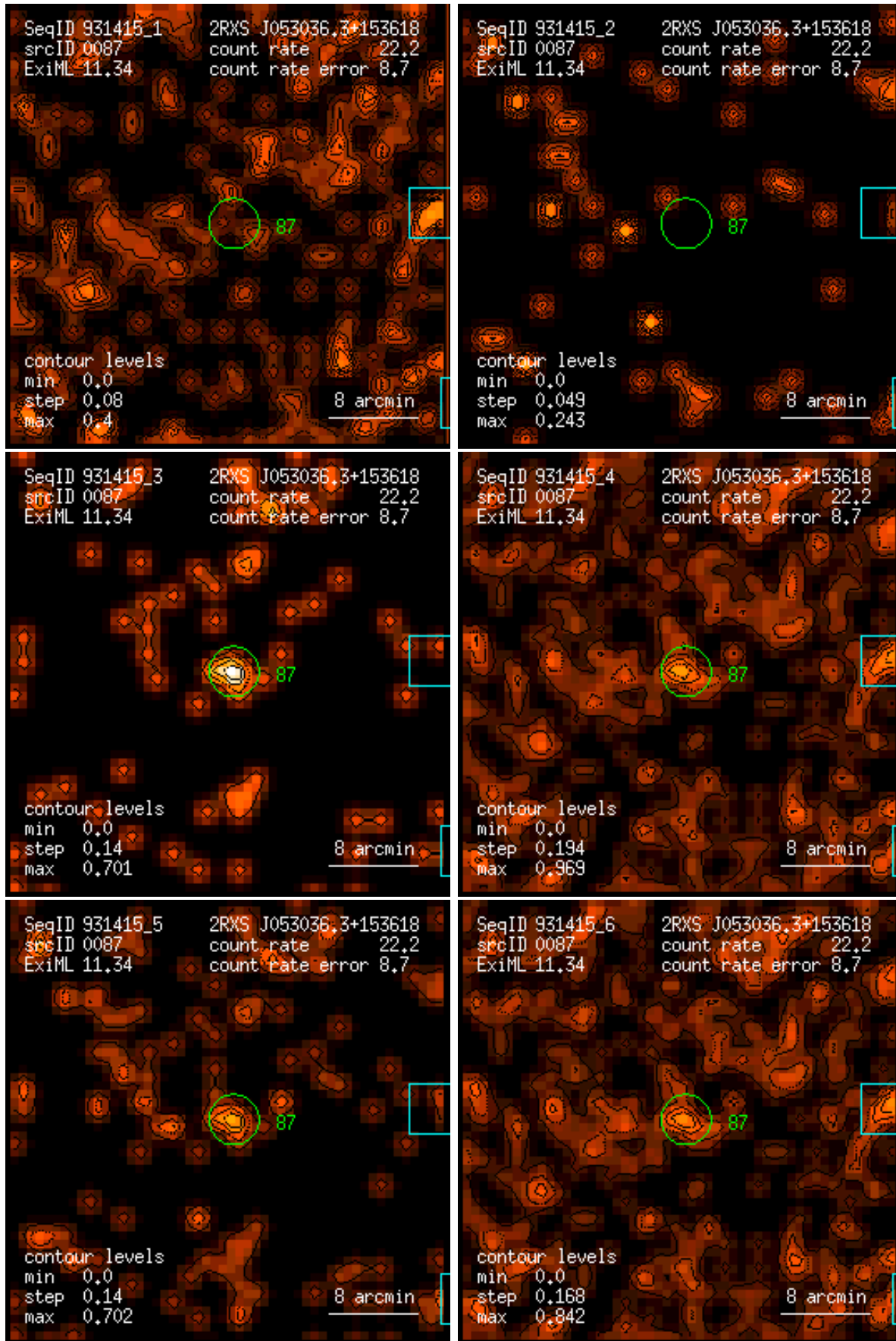
Figure 87: RASS 931415: detection 0087: band rate images, Gaussian filter: (1) PSPC channels 11 – 41, (2) 52 – 90, (3) 91 – 201, (4) 11 – 235, (5) 52 – 201, (6) 11 – 201. Broad band rates in counts/ks. Band rate contour levels in counts/ks/arcmin 2 .
