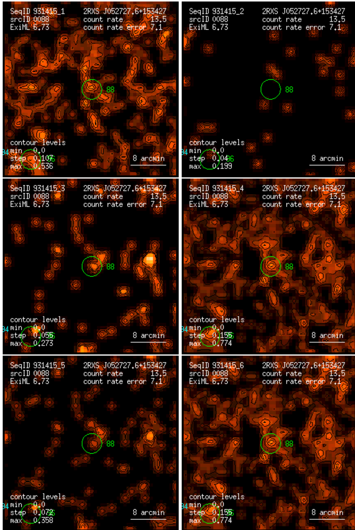
Figure 88: RASS 931415: detection 0088: band rate images, Gaussian filter: (1) PSPC channels 11 – 41, (2) 52 – 90, (3) 91 – 201, (4) 11 – 235, (5) 52 – 201, (6) 11 – 201. Broad band rates in counts/ks. Band rate contour levels in counts/ks/arcmin 2 .
