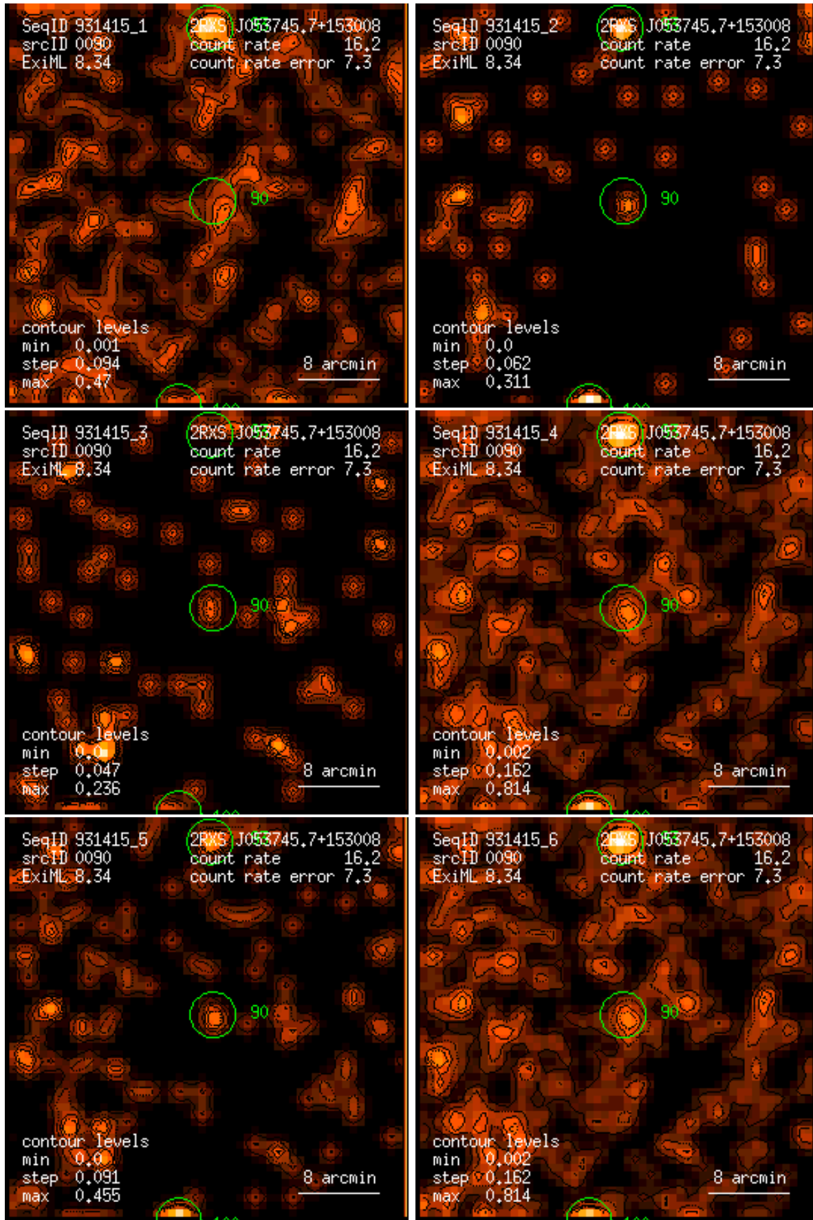
Figure 90: RASS 931415: detection 0090: band rate images, Gaussian filter: (1) PSPC channels 11 – 41, (2) 52 – 90, (3) 91 – 201, (4) 11 – 235, (5) 52 – 201, (6) 11 – 201. Broad band rates in counts/ks. Band rate contour levels in counts/ks/arcmin 2 .
