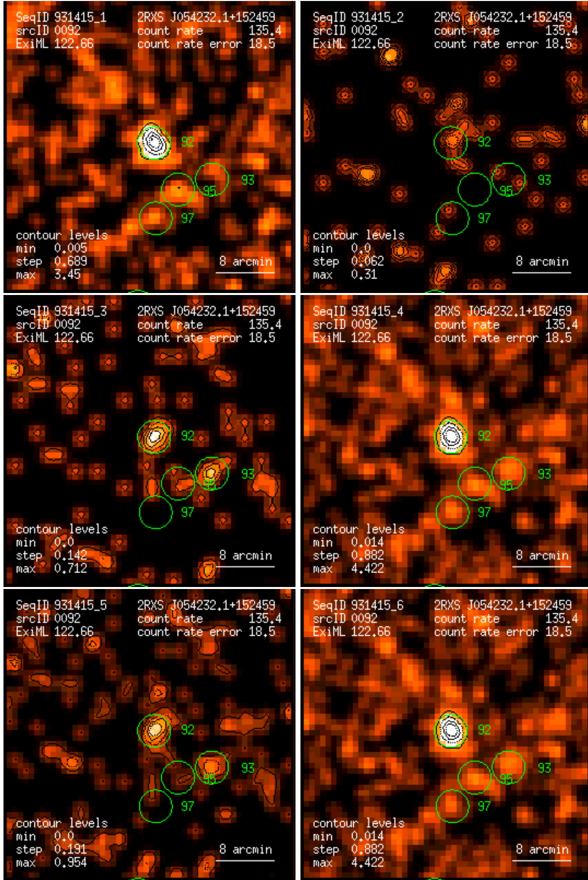
Figure 92: RASS 931415: detection 0092: band rate images, Gaussian filter: (1) PSPC channels 11 – 41, (2) 52 – 90, (3) 91 – 201, (4) 11 – 235, (5) 52 – 201, (6) 11 – 201. Broad band rates in counts/ks. Band rate contour levels in counts/ks/arcmin 2 .
