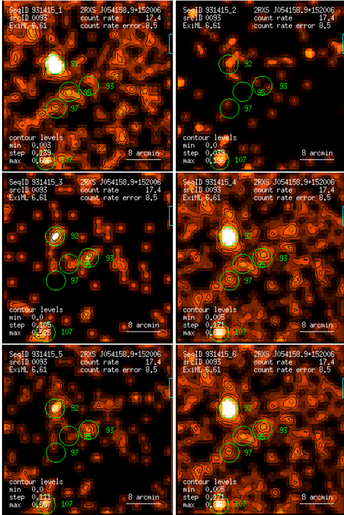
Figure 93: RASS 931415: detection 0093: band rate images, Gaussian filter: (1) PSPC channels 11 – 41, (2) 52 – 90, (3) 91 – 201, (4) 11 – 235, (5) 52 – 201, (6) 11 – 201. Broad band rates in counts/ks. Band rate contour levels in counts/ks/arcmin 2 .
