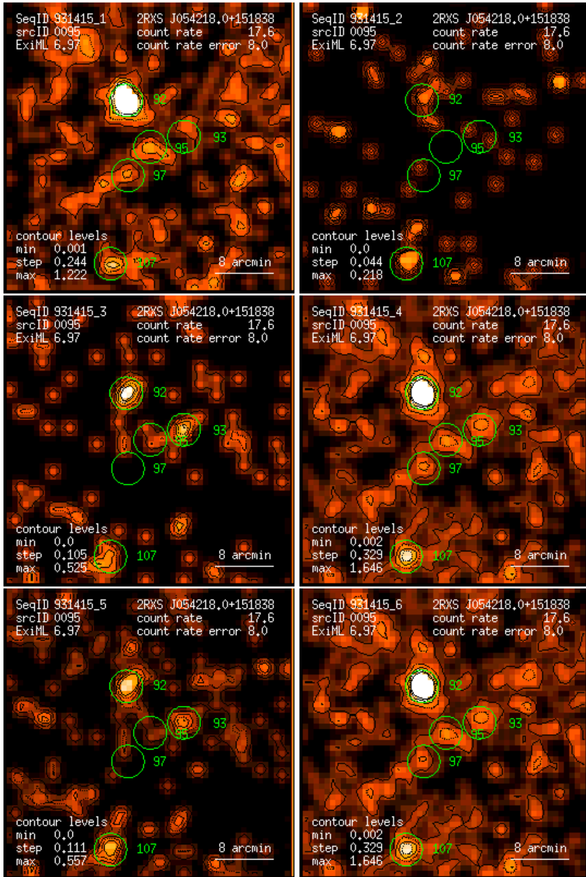
Figure 95: RASS 931415: detection 0095: band rate images, Gaussian filter: (1) PSPC channels 11 – 41, (2) 52 – 90, (3) 91 – 201, (4) 11 – 235, (5) 52 – 201, (6) 11 – 201. Broad band rates in counts/ks. Band rate contour levels in counts/ks/arcmin 2 .
