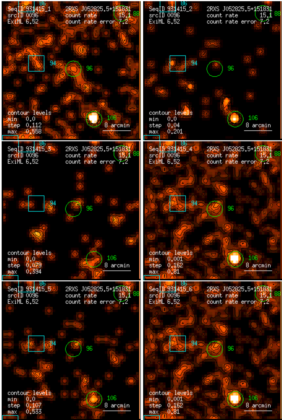
Figure 96: RASS 931415: detection 0096: band rate images, Gaussian filter: (1) PSPC channels 11 – 41, (2) 52 – 90, (3) 91 – 201, (4) 11 – 235, (5) 52 – 201, (6) 11 – 201. Broad band rates in counts/ks. Band rate contour levels in counts/ks/arcmin 2 .
